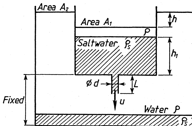
Fig.3 Model of the System
