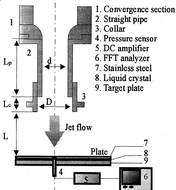
Fig. 1 Experimental apparatus.
