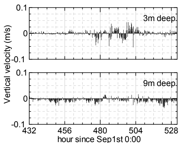
Fig. 12 Vertical velocity vectors measured by ADCP (Typhoon 2011/15)
