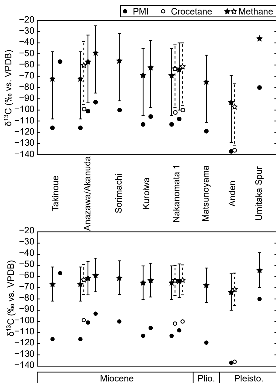
Fig. 1.7. Stable carbon isotopic compositions of the lipid biomarkers for anaerobic methane-oxidizing archaea, PMI and crocetane, extracted from the seep carbonates (filled and open circles). Stars indicate the carbon isotopic compositions of the source methane, which were estimated based on the carbon isotope offset ( \Delta\delta^{13}\text{C}_{\text{methane} - \text{lipid}} , Fig. 1.3A) in the upper panel and on the regression lines (Fig. 1.3B) in the lower panel. Filled and open stars indicate the values estimated using the isotopic compositions of PMI and crocetane, respectively. In both panels, error bars indicate the range of the estimated values. Ordered from the oldest (left) to youngest (right) site. Pleisto., Pleistocene; Plio., Pliocene.
