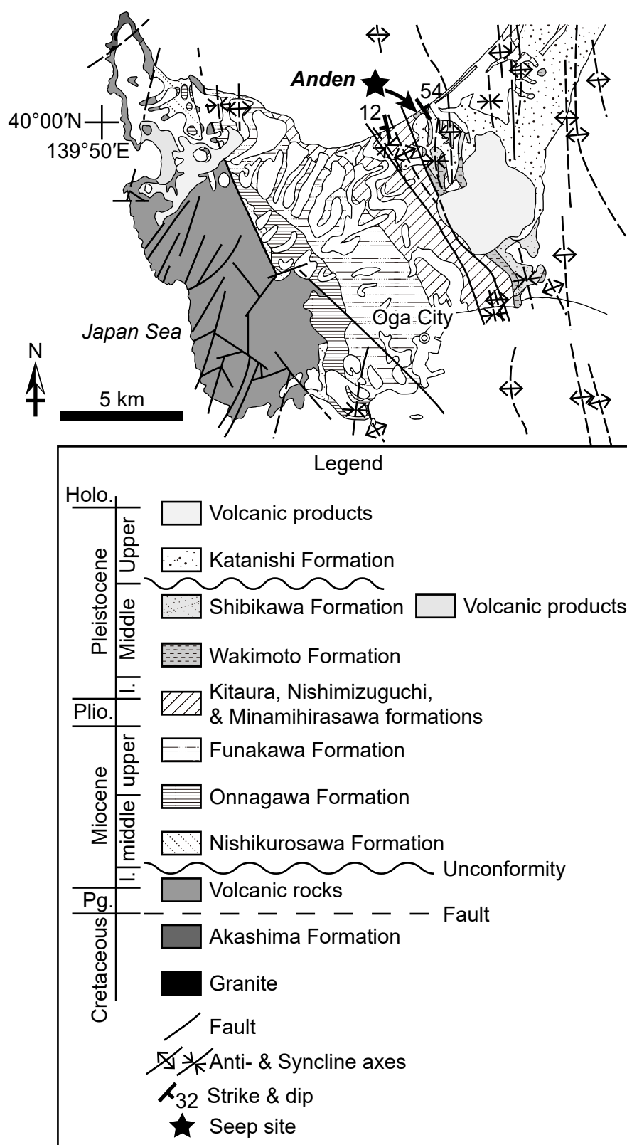
Fig. A.16. Geological map of the Oga Peninsula (modified from Kano et al., 2011).
