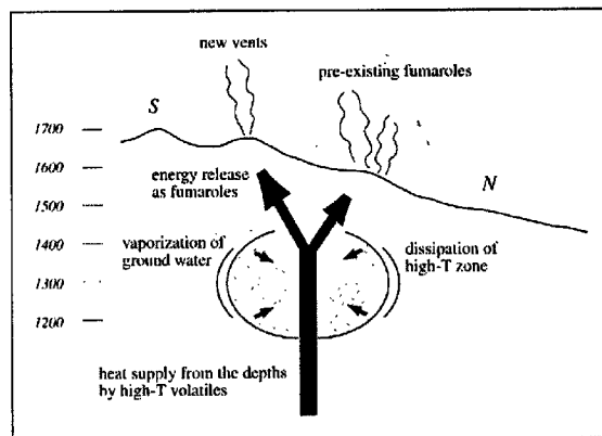
Fig. 4 Schematic image of heat discharging process of Kujū-Iwoyama as inferred from geomagnetic changes.
