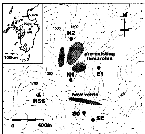
Fig. 1 Locations of geomagnetic stations (solid circles), pre-existing fumaroles and new vents on Kuju Iwoyama Volcano. Reduction is made by referring to AVL (30km SW from Kuju). HSS indicates the peak of Mt. Hossho.
