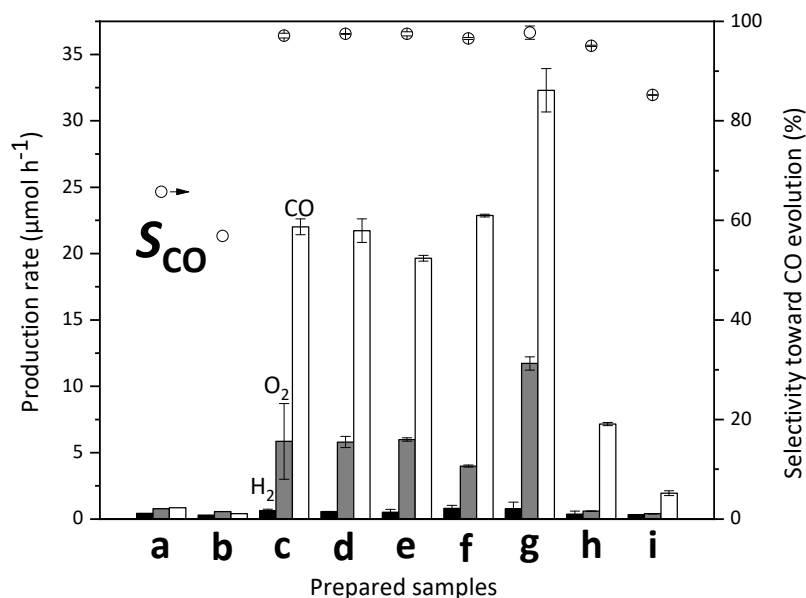
Fig. 7. Formation rates of H 2 (black), CO (white), and O 2 (gray), and the selectivity to CO ( S_{\text{CO}}\% , open circles) in the photocatalytic reaction tests for CO 2 reduction by H 2 O with (a) the bare CTO sample, (b) the Pr(1.0,773)/CTO sample, (c) the Ag(3.5)/CTO sample, and the
