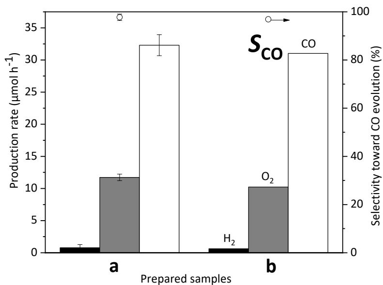
Fig. S9. Formation rates of H 2 (black), CO (white), and O 2 (gray), and the selectivity to CO ( S_{CO} %, open circles) in the photocatalytic reaction tests for CO 2 reduction with (a) the Ag(3.5)/Pr(1.0,773)/CTO sample and (b) the used Ag(3.5)/Pr(1.0,773)/CTO sample.
