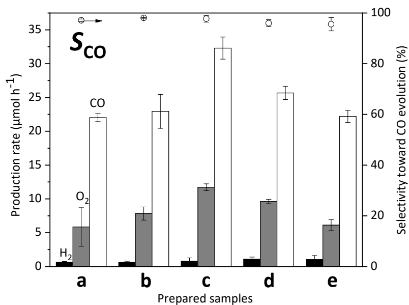
Fig. S7. Formation rates of \text{H}_2 (black), \text{CO} (white), and \text{O}_2 (gray), and the selectivity to \text{CO} ( S_{\text{CO}}\% , open circles) in the photocatalytic reaction tests for \text{CO}_2 reduction with (a) the \text{Ag}(3.5)/\text{CTO} sample and the \text{Ag}(3.5)/\text{Pr}(\gamma, 773)/\text{CTO} samples, where the \gamma wt% was (b) 0.5, (c) 1.0, (d) 1.5, and (e) 3.0.
