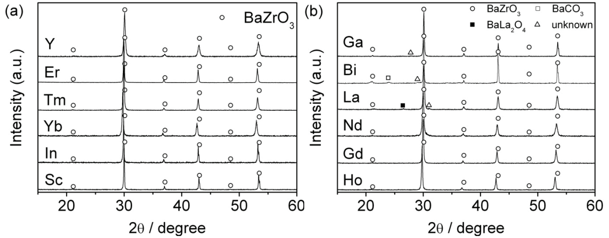
Figure 3.3 XRD patterns of pellets of X_{MO_{1.5}} = 0.075 at X_{BaO} = 0.50 after heat-treatment at 1600 °C for 24 hours ((a) M = Sc, In, Yb, Tm, Er, Y (b) M = Ho, Gd, Nd, La, Bi, Ga). Each symbol indicates diffraction patterns of ○ ( BaZrO_3 , JCPDS No. 00-006-0399), □ ( BaCO_3 , JCPDS No. 00-005-0378), ■ ( BaLa_2O_4 , JCPDS No. 00-042-1500) and Δ (unknown peak).
