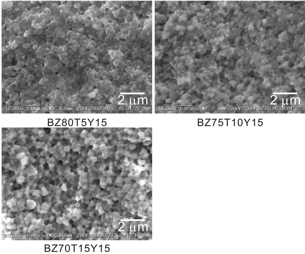
Figure 8.7 Cross-sectional SEM images of BZ80T5Y15, BZ75T10Y15 and BZ70T15Y15.
