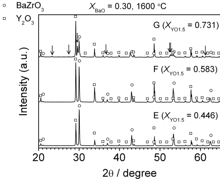
Figure 4.4 XRD patterns of samples at X_{\text{BaO}} = 0.30 after heat-treating at 1600^\circ\text{C} for 24 hours ((a) sample A to D, (b) sample E to G). Each symbol indicates diffraction patterns of ○ ( \text{BaZrO}_3 , JCPDS No. 00-006-0399), △ ( \text{ZrO}_2 , JCPDS No. 00-027-0997) and □ ( \text{Y}_2\text{O}_3 , JCPDS No. 00-043-1036).
