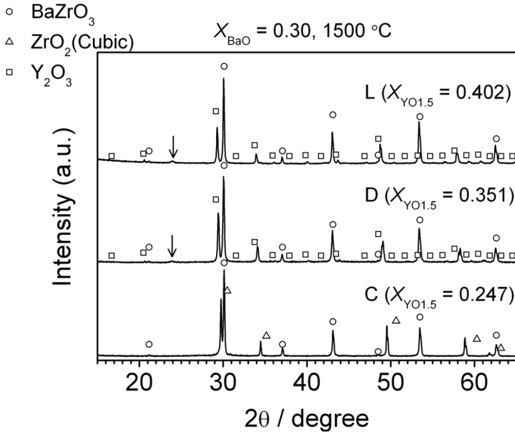
Figure 4.9 XRD patterns of samples at X_{\text{BaO}} = 0.30 after heat-treating at 1500\text{ }^\circ\text{C} for 100 hours ((a) X_{\text{YO}_{1.5}} = 0.247, 0.351 and 0.402 ). Each symbol indicates diffraction patterns of ○ ( \text{BaZrO}_3 , JCPDS No. 00-006-0399), △ ( \text{ZrO}_2 , JCPDS No. 00-027-0997), □ ( \text{Y}_2\text{O}_3 , JCPDS No. 00-043-1036).
