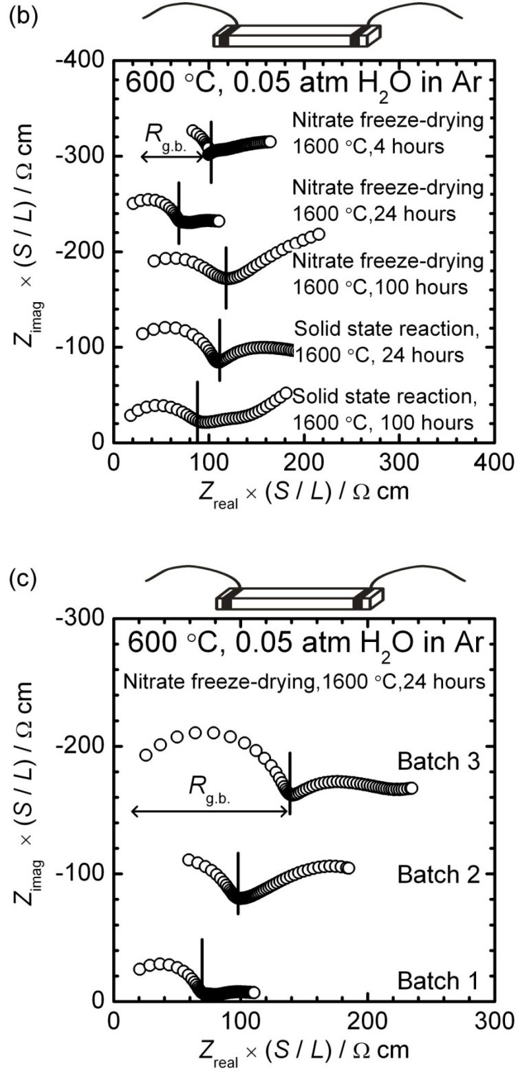
Figure 9.7 AC 2-terminal impedance spectra in Ar-0.05 % H 2 O of BaZr 0.85 Y 0.15 O 3-δ at (a) 80 °C using pellets, (b) 600 °C using bars and (c) comparison of AC 2-terminal impedance spectra of three batches of BaZr 0.85 Y 0.15 O 3-δ sintered for 24 hours at 1600 °C from powders obtained by using nitrate freeze-drying method and synthesis at 500 °C for 10 hours. The sintering time and synthesis method are indicated in the figure.
