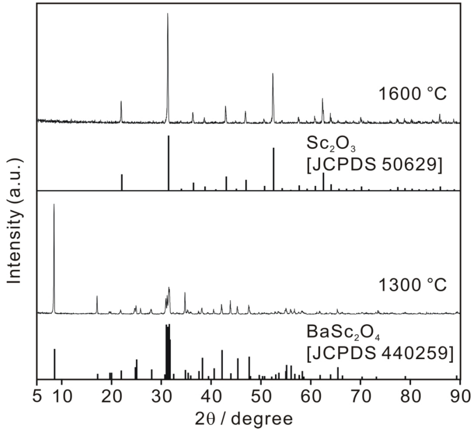
Figure 5.5 XRD patterns of \text{BaSc}_2\text{O}_4 at 1300 °C and 1600 °C.
