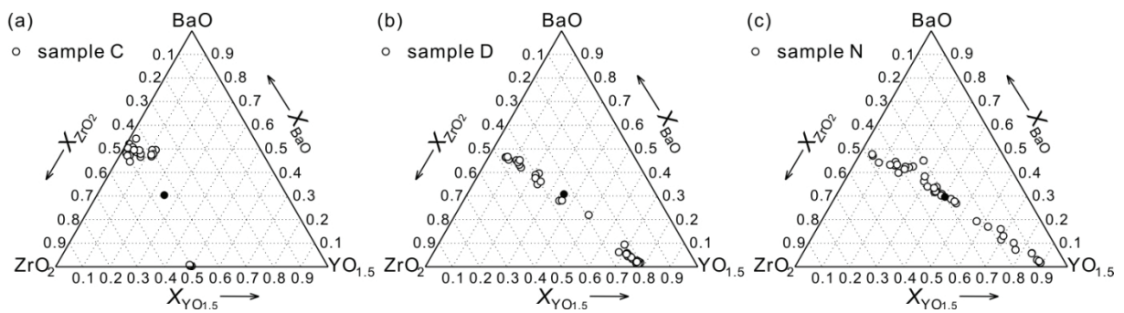
Figure 4.10 Results of EDX analysis in samples after heat-treating at 1500\text{ }^\circ\text{C} for 100 hours on pseudoternary phase diagrams of \text{BaO-ZrO}_2\text{-MO}_{1.5} system ((a) sample C, (b) sample D, (c) sample N). Black point is an average composition of each sample.
