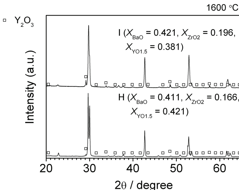
Figure 4.7 XRD patterns of sample H and I after heat-treatment at 1600 °C for 24 hours. Each symbol indicates diffraction patterns of \square ( \text{Y}_2\text{O}_3 , JCPDS No. 00-043-1036).
