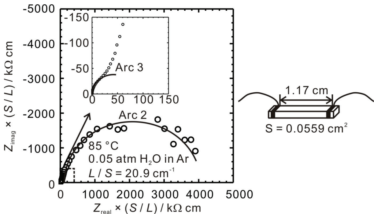
Figure 2.8 AC 2-terminal impedance spectrum at 85\text{ }^{\circ}\text{C} in \text{Ar}-0.05\text{ }\%\text{H}_2\text{O} using a bar of \text{BaZr}_{0.85}\text{Y}_{0.15}\text{O}_{3-\delta} .
