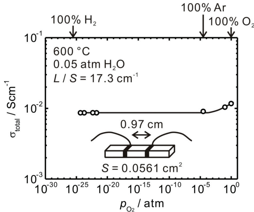
Figure 2.10 Dependence of oxygen partial pressure on total conductivity of \text{BaZr}_{0.85}\text{Y}_{0.15}\text{O}_{3-\delta} at 600 °C in 0.05 % \text{H}_2\text{O} .
