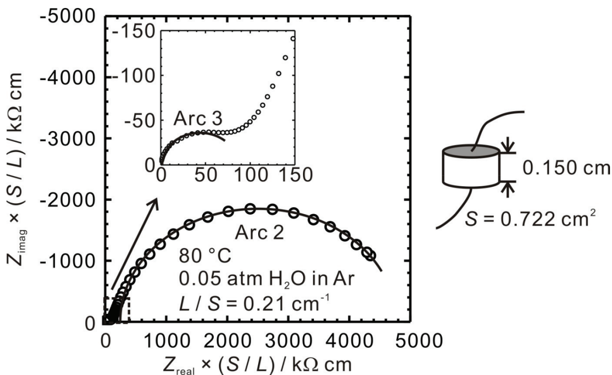
Figure 2.9 AC 2-terminal impedance spectrum at 80\text{ }^{\circ}\text{C} in \text{Ar}-0.05\text{ }\%\text{H}_2\text{O} using a pellet of \text{BaZr}_{0.85}\text{Y}_{0.15}\text{O}_{3-\delta} .
