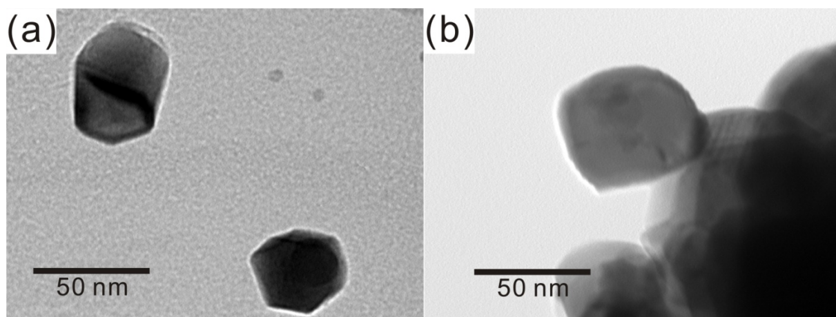
Figure 9.5 TEM image of \text{BaZr}_{0.85}\text{Y}_{0.15}\text{O}_{3-\delta} powders (a) obtained by nitrate freeze-drying method and synthesis at 500 °C for 10 hours in vacuum and (b) obtained by solid state reaction method at 1300 °C for 10 hours in air and ball-milling for 100 hours.
