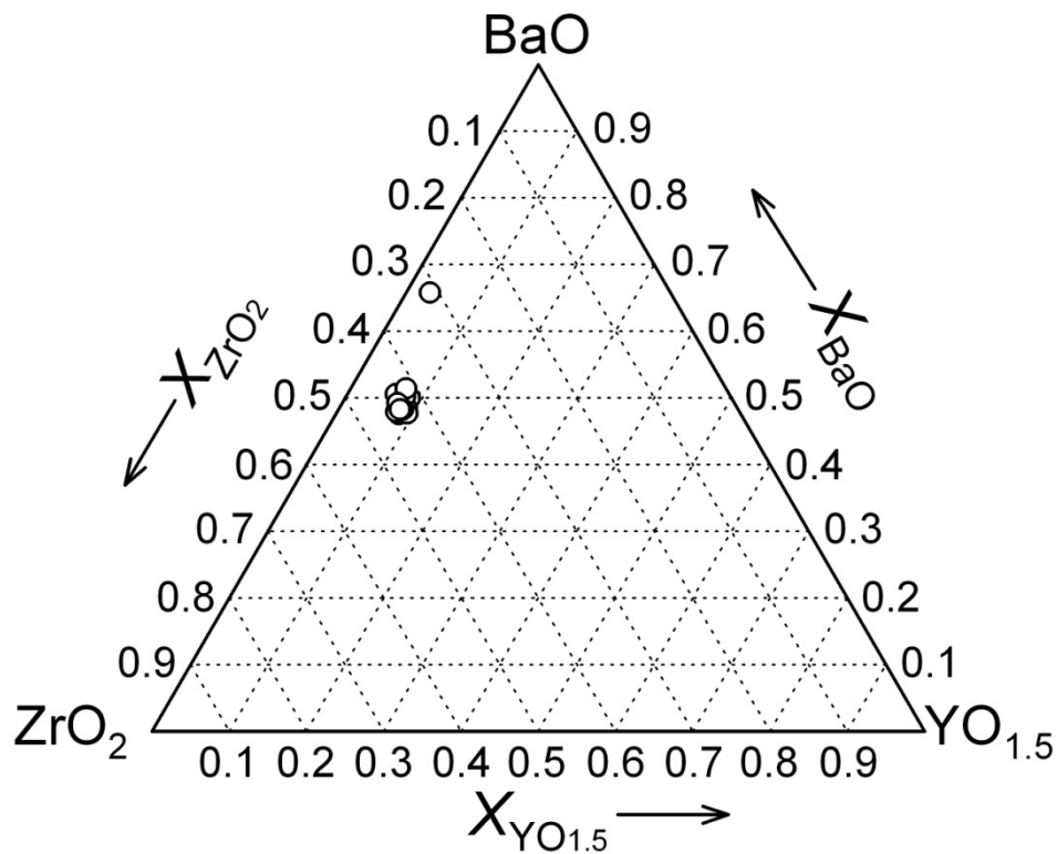
Figure 6.7 (b) The compositions of grains in the pellet on pseudoternary phase diagrams of \text{BaO} - \text{ZrO}_2 - \text{YO}_{1.5} system.
