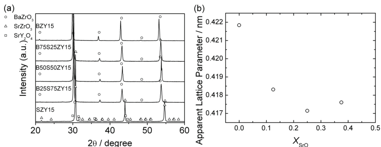
Figure 8.10 (a) XRD patterns of pellets of BZY15, B75S25ZY15, B50S50ZY15, B25S75ZY15 and SZY15 after heat-treatment at 1600 °C for 24 hours. Each symbol indicates diffraction patterns of \circ ( \text{BaZrO}_3 , JCPDS No. 60399), \Delta ( \text{SrZrO}_3 , JCPDS No. 00-044-0161) and \square ( \text{SrY}_2\text{O}_4 , JCPDS No. 00-032-1272). (b) Apparent lattice parameters of barium zirconate phase as a function of the mole fraction of strontium oxide, X_{\text{SrO}} .
