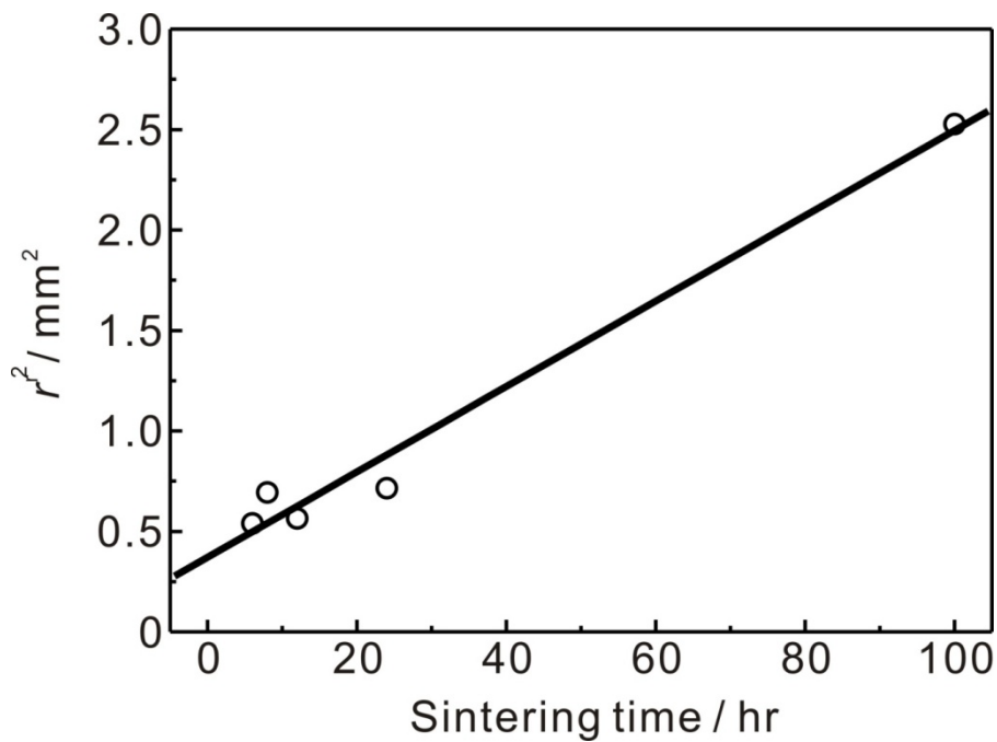
Figure 6.5 Average square grain sizes of \text{BaZr}_{0.85}\text{Sc}_{0.15}\text{O}_{3-\delta} sintered in air as a function of sintering time.
