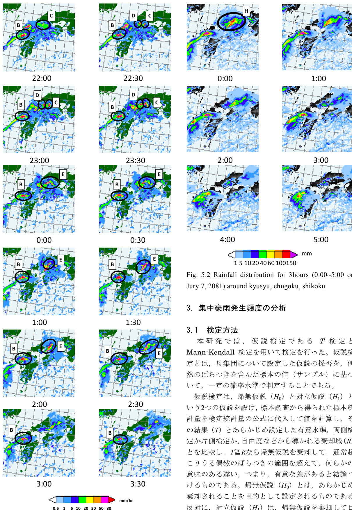
Fig. 4.2 Rainfall distribution for 30 minutes(22:00 on July 6~3:30 on July 7, 2081) around kyusyu, chugoku, shikoku
