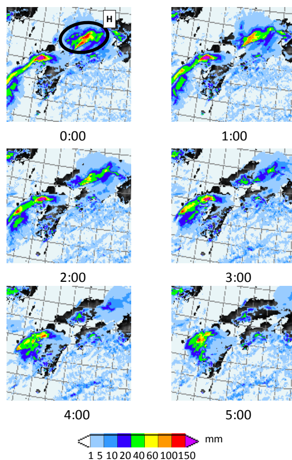
Fig. 5.2 Rainfall distribution for 3hours (0:00~5:00 on July 7, 2081) around kyusyu, chugoku, shikoku
