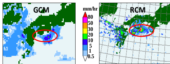
Fig. 2 20kmGCM(left) and 5kmRCM(right)
