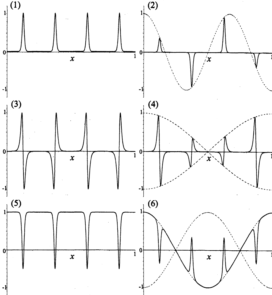
Figure 5: Graphs of eigenfunctions for case f(u) = u(1 - u^2) ( n = 4 and k = 1 - 10^{-10} ): (1) \varphi_0^4(x; k) , (2) \varphi_3^4(x; k) , (3) 2\varphi_4^4(x; k) , (4) 2\varphi_5^4(x; k) , (5) \varphi_8^4(x; k)/2 , (6) \varphi_{10}^4(x; k)/2 .
