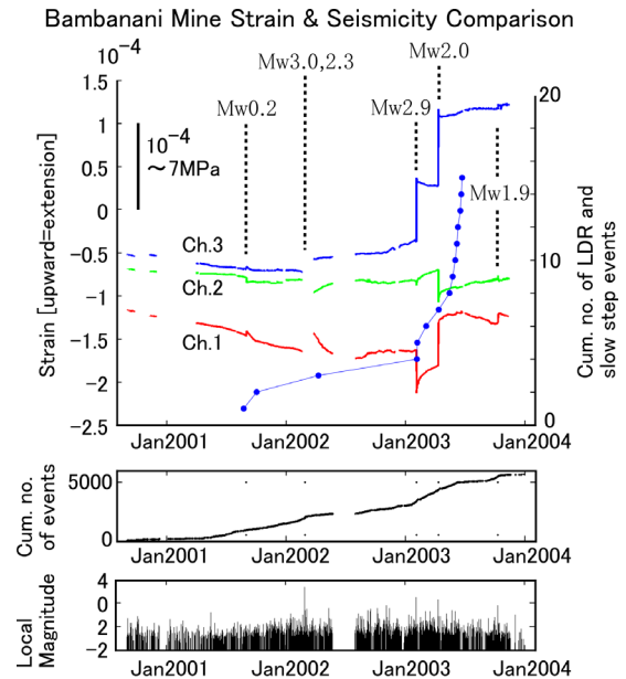
Figure 2. Long-term strain changes and seismicity within 250m of our strainmeter at the Bambanani mine (after Ogasawara et al. [2005]), and the occurrence of LDR (Little Dynamic Response) events, which is central in this article, as detailed in Section 3, with steps of > 10^{-7} . Connected blue dots show cumulative number of LDR events highlighted in this study. LDR events frequently occur after the onset of large strain changes, except for the event of August 2001 prior to the Mw0.2 earthquake in September 2001.
