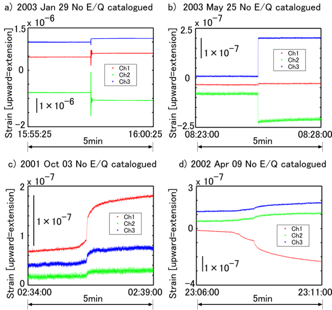
Figure 3. Examples of strain events in 5-minute periods (a) with dynamic strain change, (b) with static strain change only, (c) slow-step with forerunner (see Figure 6b for different time scales), and (d) slow-step (see Figure 6b for different time scales).
