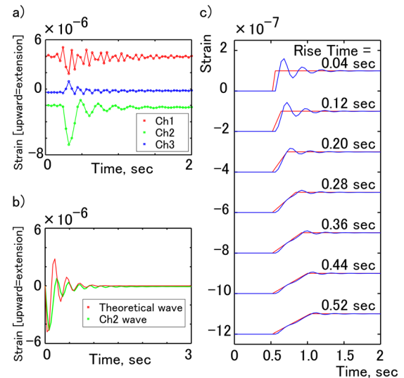
Figure 6. The change in DR with an increasing duration of the step rise-time. (a) An example of observed DR (for a 2-second period; Mw = 0.1 max. step = 2.2 \times 10^{-7} on 2002 Aug. 1), (b) Ch 2 strain changes and approximated damped oscillation, and (c) synthesized strain steps for variable rise times from 0.04 to 0.52 second.
