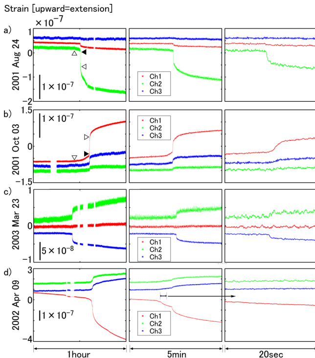
Figure 5. Four examples of slow-step events. Open triangles are onsets of forerunner and post-seismic drift. Solid triangles are onsets of co-seismic steps.
