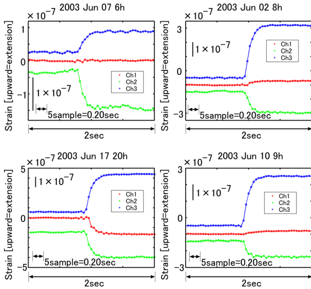
Figure 4. Four examples of LDR events with little impulse and step responses.
