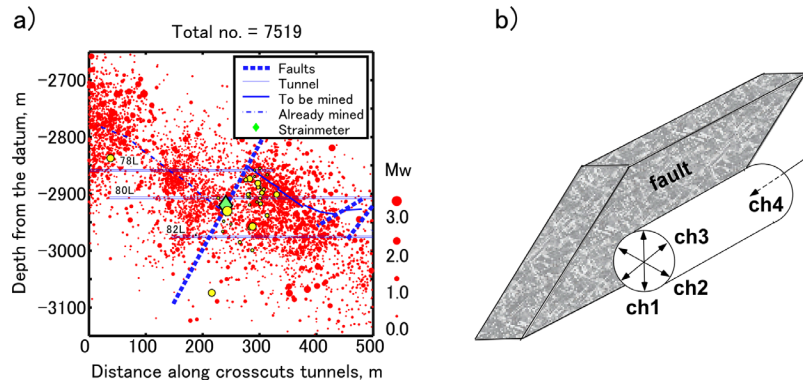
Figure 1. (a) Seismicity within 400m of the strainmeter ( -0.5 < M_w < 3 ; detected at more than four stations; from June 2001 to June 2003; vertical cross section; data supplied by the mine). Yellow-circle; earthquakes with strain steps > 10^{-7} . The location accuracy is relatively low in a direction normal to the reef along the fault because the station configuration is almost planar along the reef [Shimoda et al. , 2005]. (b) Schematic illustration of normal fault and configuration of sensor directions in the Ishii strainmeter.
