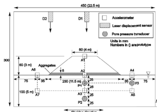
Fig. 1. Model configuration in rigid container.
