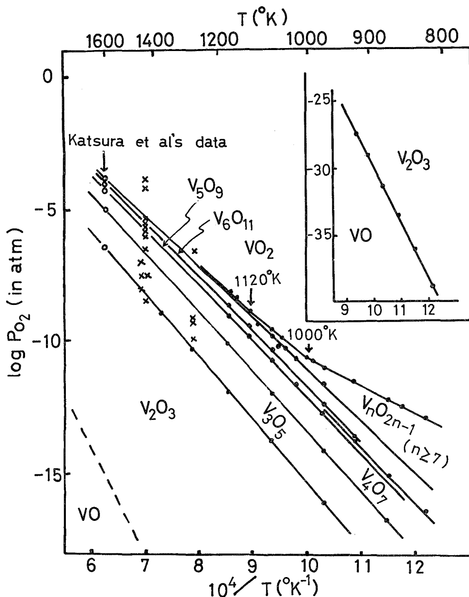
Fig. 1. Plot of \log P_{O_2} versus 10^4/T (°K -1 ) for the V_2O_3 , V_3O_5 , V_4O_7 , V_5O_9 , V_6O_{11} , V_7O_{13} and VO_2 respectively. 8)
