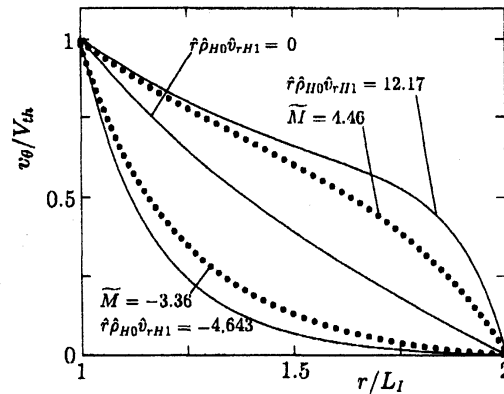
FIG. 8: Profiles of the tangential velocity v_{\theta} at \text{Kn} = 0.005 (DSMC result for hard-sphere molecules) corresponding to (V_I/V_{th}, \tilde{M}) = (1.0053, -3.36) and (1.0053, 4.46) in the case of n_{av}^B/n_I = 0.05 , n_{II}/n_I = 1.5 , m^B/m^A = 1 , and d^B/d^A = 1 ( L_{II}/L_I = 2 , T_{II}/T_I = 1 , and V_{II} = 0 ). The corresponding results in the continuum limit, i.e., the profiles at (V_I/V_{th}, \hat{r}\hat{\rho}_{H0}\hat{v}_{rH1}) = (1.0053, -4.643) , (1.0053, 0) , and (1.0053, 12.17) , are also shown by the solid line.
