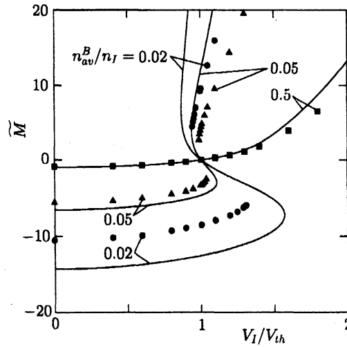
FIG. 7: Magnified mass flow rate \tilde{M} versus V_I/V_{th} at \text{Kn} = 0.005 (DSMC result for hard-sphere molecules) for n_{av}^B/n_I = 0.5, 0.05 , and 0.02 in the case of n_{II}/n_I = 1.5 , m^B/m^A = 1 , and d^B/d^A = 1 ( L_{II}/L_I = 2 , T_{II}/T_I = 1 , and V_{II} = 0 ). The solid line indicates the results in the continuum limit.
