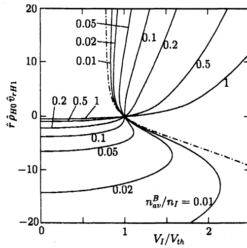
FIG. 5: The \hat{r} \hat{\rho}_{H0} \hat{v}_{rH1} versus V_I/V_{th} in the continuum limit for various n_{av}^B/n_I (hard-sphere molecules) in the case of n_{II}/n_I = 1.5 , m^B/m^A = 1 , and d^B/d^A = 1 ( L_{II}/L_I = 2 , T_{II}/T_I = 1 , and V_{II} = 0 ). The dot-dashed line indicates the pure vapor case [12].
