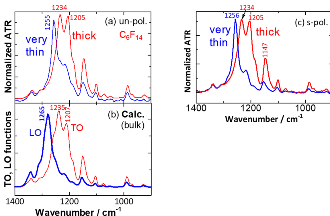
FIG. 5. Comparison of (a) the observed ATR spectra of C_6F_{14} with (b) the calculated bulk TO and LO functions. (c) The s-polarization spectra reproduce the un-polarized spectra.
