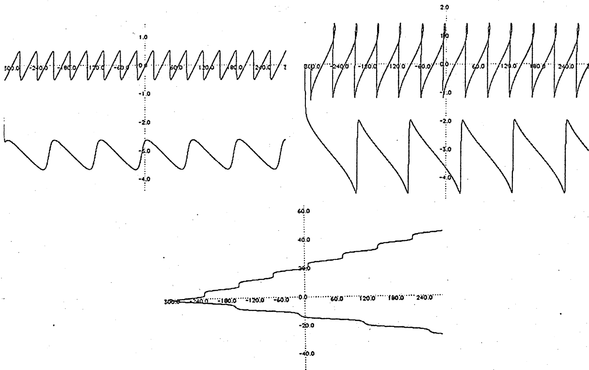
Figures 4a,b,c. Trajectories (X, Y) from (8), for K = 0.5, 1.0 and 1.5 respectively, with \sigma = 0.5 and \varepsilon = 0.1 . Upper curves are growing modes, and lower curves decaying modes.
