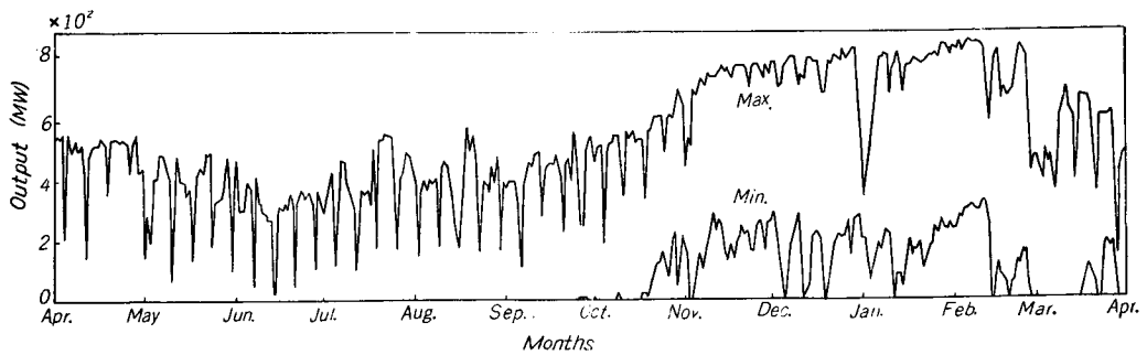
Fig. 1. Daily maximum and minimum output of the steam-power in a system
