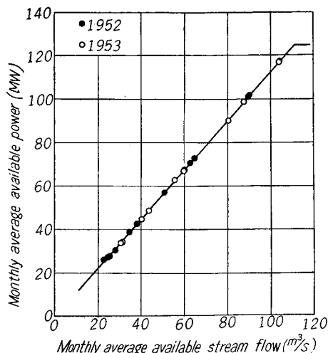
Fig. 9. The relation between the monthly average available power and stream flow
