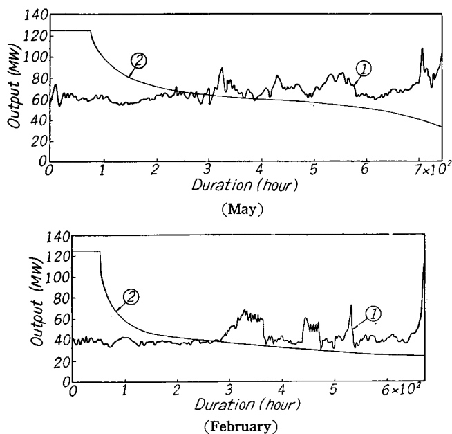
Fig. 7. Vertical distance between the monthly duration curve of the total load of a system and that of the residual load after the completion of a run-off-river hydro-power
