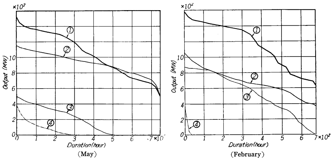
Fig. 3. Monthly duration curves of a system
