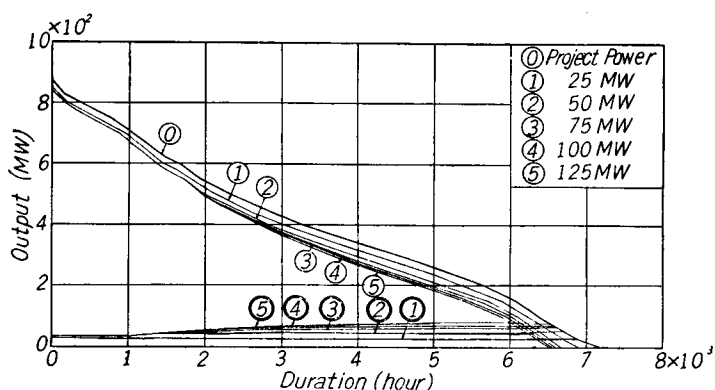
Fig. 6. Annual duration curves of the total load of a system and the residual load after the completion of a newly projected run-off-river hydro-power
