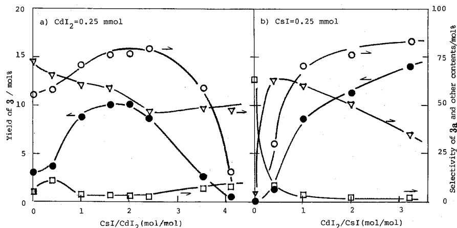
Fig. 1. Effect of ratio of charge mole ratio CsI/CdI 2 and CdI 2 /CsI. Conditions: K 2 -phthalate( 2b )=2 mmol, Naphthalene( 1 )=20 mmol, K 2 -phthalate ( 2b )=2 mmol, CO 2 =80 atm, 400°C, 2.5h. ●: yield of 3 (based on the charged 2b ), ○: Selectivity of 3a , ▽: 2c , □: 2a .
