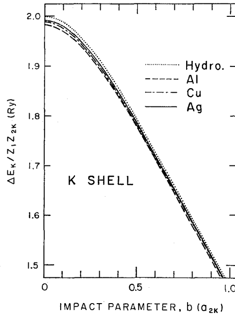
Fig. 1. The increase in scaled binding energy of K shell, \Delta E_K/Z_1 Z_{2K} , as a function of impact parameter for aluminum, copper, and silver. The dotted line represents the results by the screened hydrogenic wave function.
