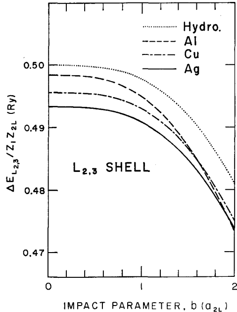
Fig. 3. The increase in scaled binding energy of L_{2,3} shell, \Delta E_{L_{2,3}}/Z_1 Z_{2L} , as a function of impact parameter for aluminum, copper, and silver. The dotted line represents the results by the screened hydrogenic wave function.
