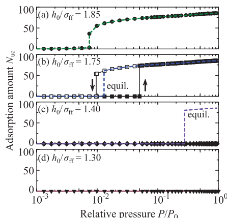
FIG. 3. Adsorption isotherms of models with initial interlayer widths h_0/\sigma_{\text{ff}} of (a) 1.85 , (b) 1.75 , (c) 1.40 , and (d) 1.30 . Filled and open symbols indicate adsorption and desorption isotherms, respectively. Dashed lines are adsorption isotherms at thermodynamic equilibrium. An interaction parameter \varepsilon_{\text{ss}}/k_B of 28\text{ K} was used for all the models.
