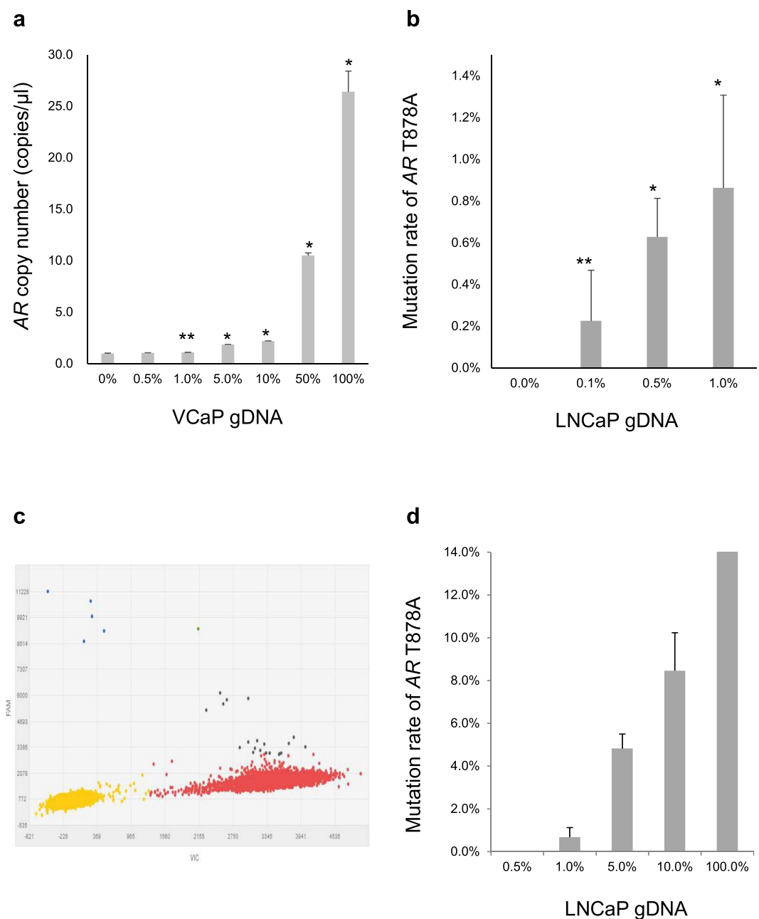
Figure 1. The sensitivity of copy number (CN) and mutation analysis by digital PCR (dPCR) and target sequencing. (a) LNCaP (AR CN neutral) genomic DNA (gDNA) was spiked with VCaP (AR amplified) gDNA in serial dilution. AR amplification could be detected by dPCR even when VCaP gDNA was diluted to 1.0%. Stars ( p < 0.01^* and p = 0.015^{**} ) indicate that AR CN in diluted VCaP gDNA are significantly higher than that in LNCaP gDNA by the Student's t-test ( n = 3 ). (b) gDNA from healthy males (AR wild type) was spiked with LNCaP (AR T878A mutated) gDNA in serial dilution. The AR T878A mutation could be detected at 0.1% dilution by dPCR. Stars ( p < 0.01^* and p = 0.014^{**} ) indicate that the mutation rates in diluted LNCaP gDNA were significantly higher than those observed in gDNA from healthy males by the Student's t-test ( n = 3 ). (c) Scatter plots of dPCR analysis for the gDNA from healthy males spiked with 0.1% LNCaP gDNA. The mutation detection rate was 0.09%. The blue dots show positive droplets for the AR T878A mutation. The red dots show positive droplets for the AR wild type. The yellow dots show empty droplets. (d) AR target sequencing for gDNA from healthy males spiked with LNCaP gDNA in serial dilution. AR T878A mutation could be detected up to 1.0% dilution. All error bars indicate standard deviation.
