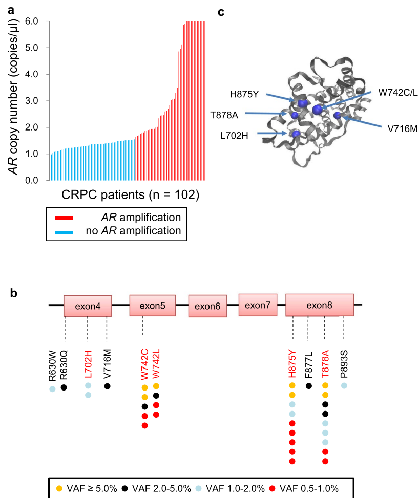
Figure 2. Landscapes of AR copy number (CN) and mutations in cfDNA from patients with CRPC (n = 102) at baseline. (a) AR amplification was defined as AR CN > 1.54 copies/μl based on AR CN in cfDNA from healthy males. The red lines show the cases with AR amplification, and the blue lines show the cases with no AR amplification. (b) The locations of the mutations identified are mapped on the AR gene. Each colored circle represents a single mutation in a single sample. The red letters indicate the known hotspots on ligand binding domain (LBD). (c) Structured 3D image of an AR protein showing that V716M is located in the proximity of the known hotspots in LBD. VAF, variant allele frequency.
