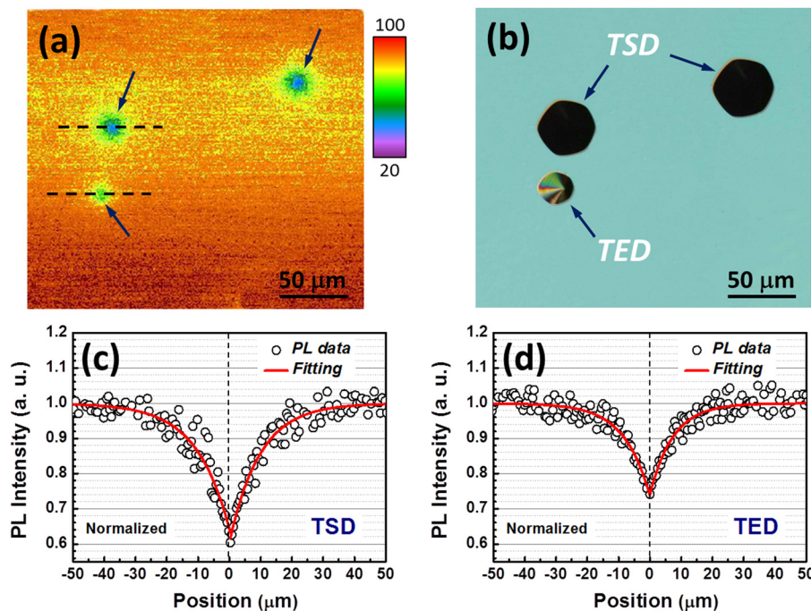
FIG. 2. (Color online) (a) \mu -PL intensity mapping at 390 nm for a 72 \mu\text{m} -thick 4H-SiC epilayer after two-step thermal treatment. (b) Surface morphology after KOH etching (the same location). (c) PL intensity profile around a TSD shown in (a). (d) PL intensity profile around a TED shown in (a).
