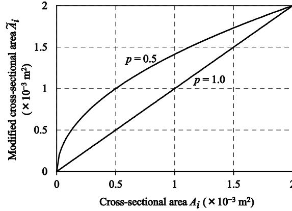
Figure 4 Relation between cross-sectional area A_i and modified cross-sectional area \tilde{A}_i
