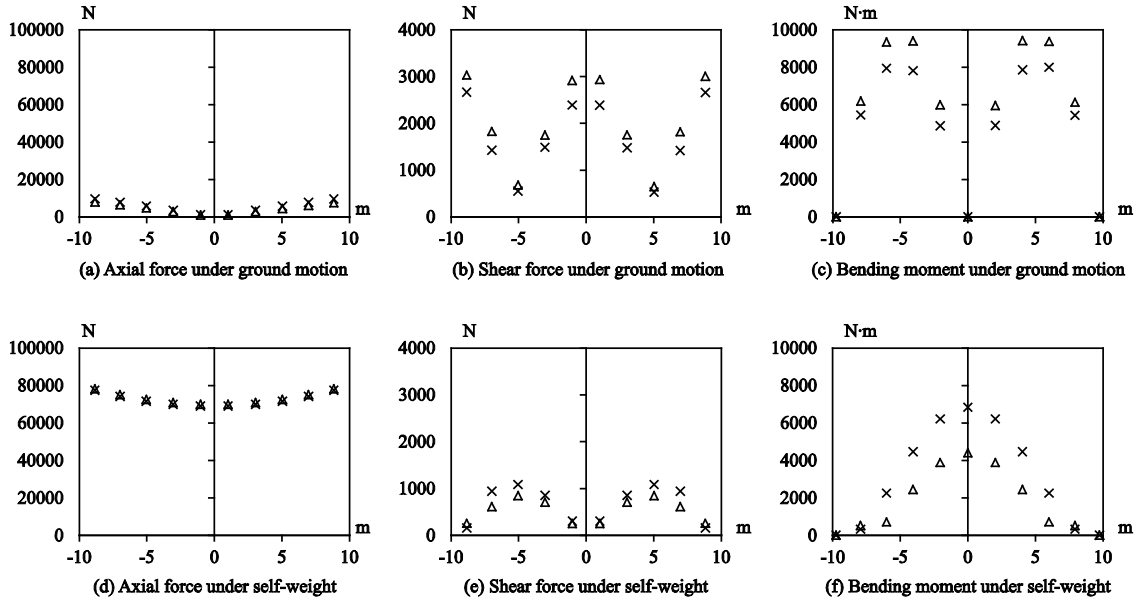
Figure 15 Mean-maximum cross-sectional forces of roof members; Δ: Stiff-model, x:Flexible-model
