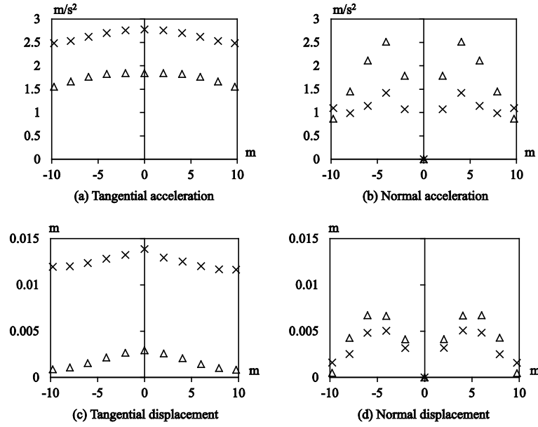
Figure 14 Mean-maximum responses of the acceleration and displacement; Δ: Stiff-model, x:Flexible-model
