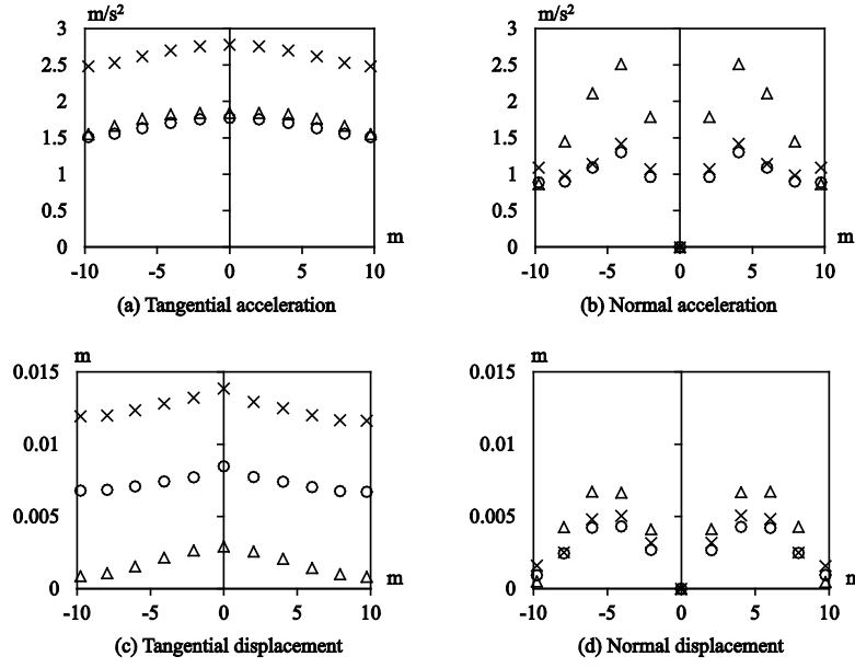
Figure 18 Mean-maximum acceleration and displacement responses; \circ : Flexible-model with dampers, \times : Flexible-model without dampers, \Delta :Stiff-model
