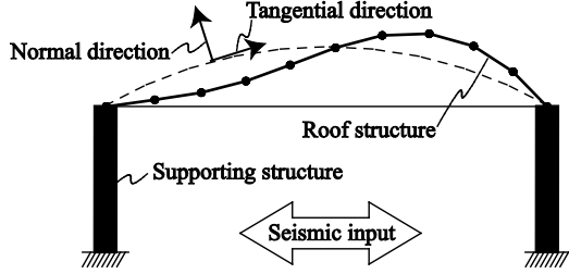
Figure 1 An arch with a conventional stiff supporting structure; solid line: deformed shape, dashed line: initial shape
