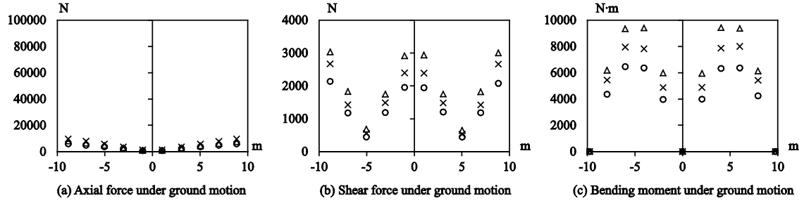
Figure 19 Mean-maximum cross-sectional forces of roof members; \circ : Flexible-model with dampers, \times : Flexible model without dampers, \Delta :Stiff-model
