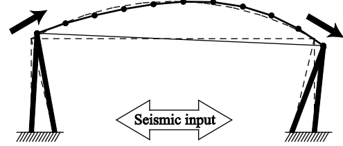
Figure 2 An arch with a flexible supporting structure; solid line: deformed shape, dashed line: initial shape
