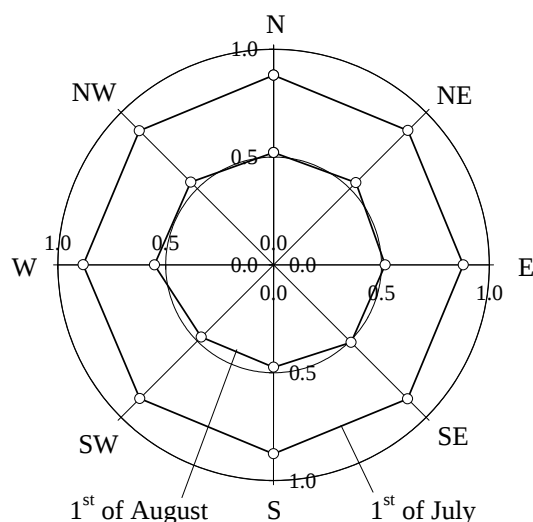
Fig. 12 Dependence of slope instability on soil moisture conditions, where minimum factor of stability on 11 th of March are adjusted to be 1.0
