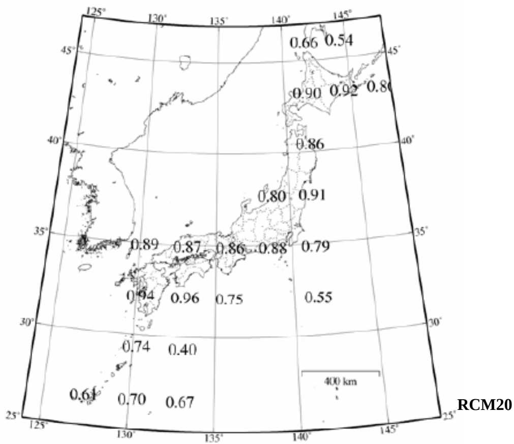
Figure 7 Coefficient of Correlation for Monthly Average Precipitation (CGCM2 and RCM20)
