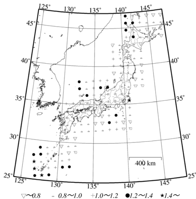
(1) Ratio of 2031-2050 to 1981-2000
