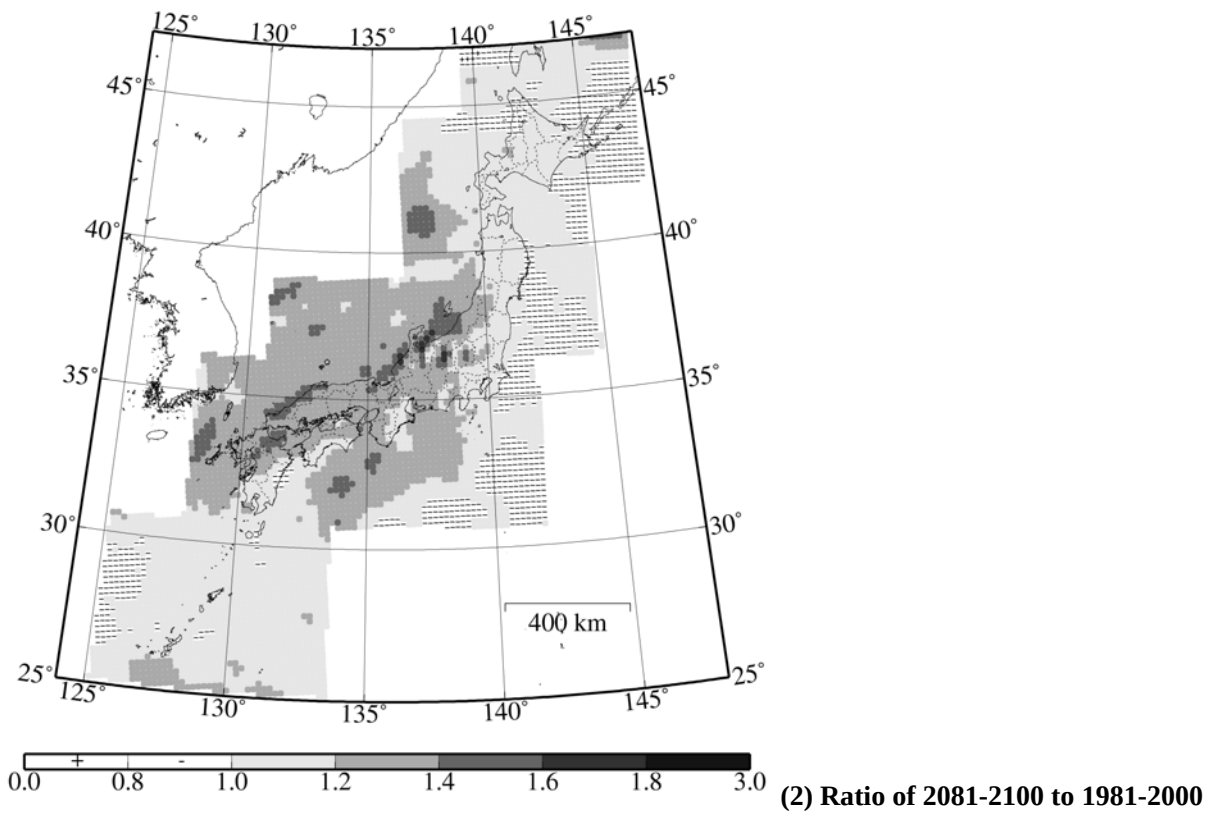
Figure 19 Comparison of Summer Precipitation
