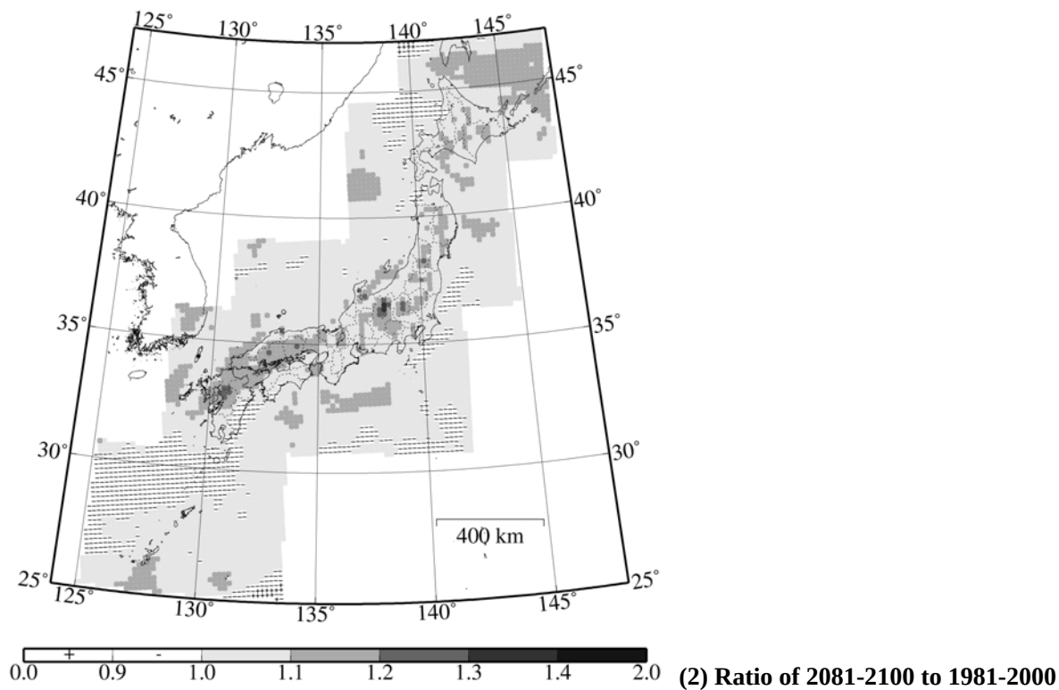
Figure 17 Comparison of Annual Precipitation
