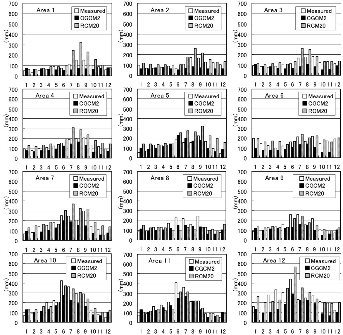
Figure 8 Monthly Average Precipitation (Observation, CGCM2 and RCM20)
