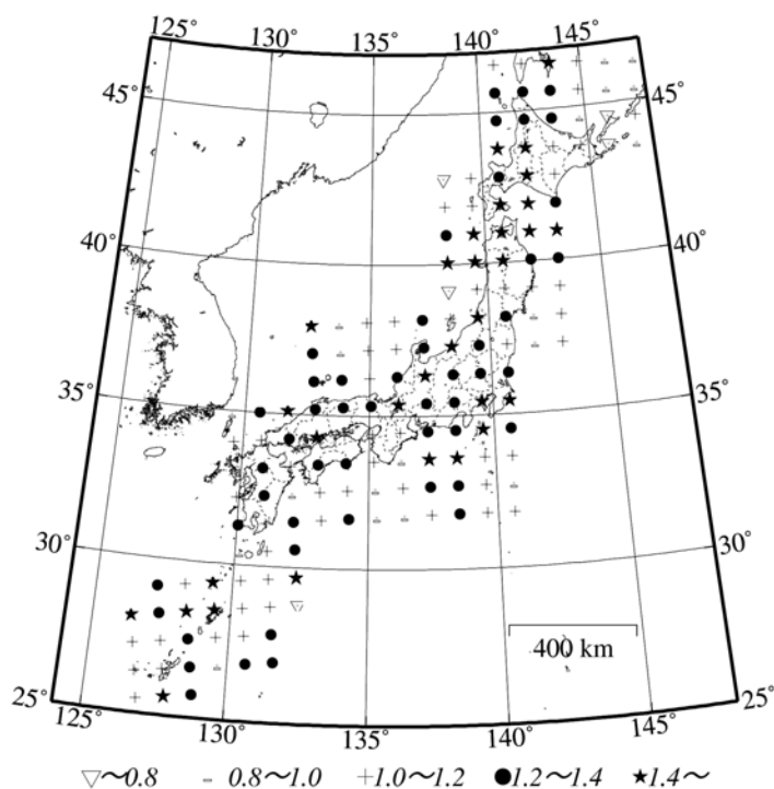
(2) Ratio of 2081-2100 to 1981-2000
