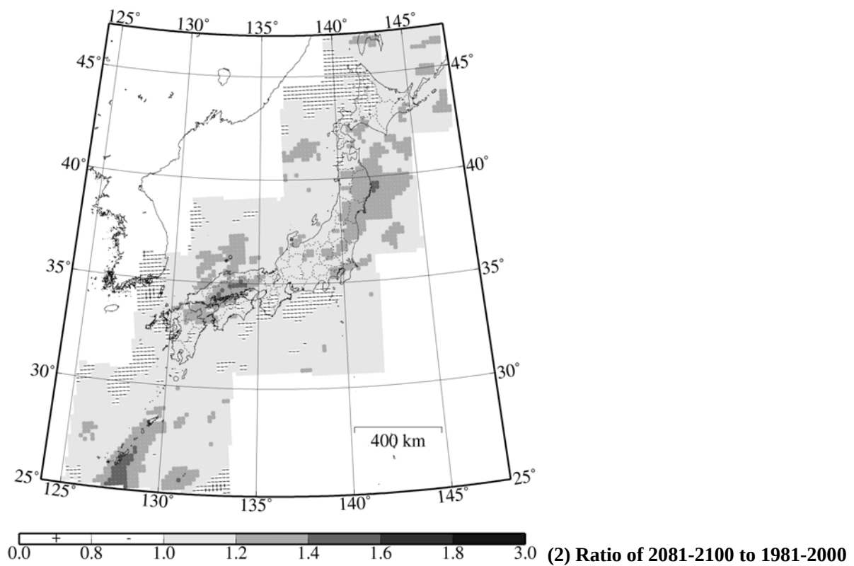
Figure 20 Comparison of Autumn Precipitation
