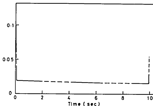
Fig. 3.2.4 Suboptimum and optimum trajectories of the neutron density for r = 0.4 .
