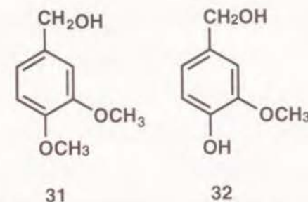
Figure 5.4 Lignin model compounds used in this experiment
