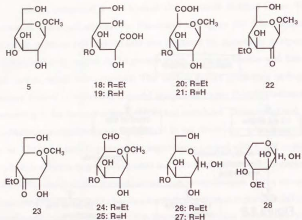
Figure 3.7 Reaction products from ozonation of methyl 4-O-ethyl-β-D-glucoside
