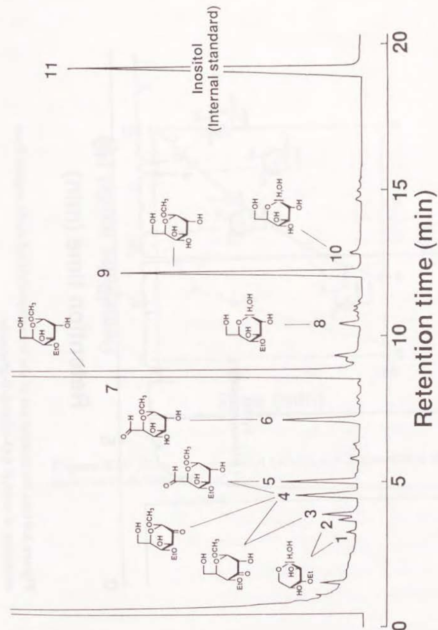
Figure 3.8 Gas chromatogram of the acetylated O-methylloximes of neutral sugars from ozonation of methyl 4-O-ethyl-β-D-glucoside.
