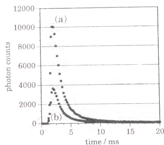
Fig. 6 Decay curves of emission by E(0.1 wt%). (a) in vacuo and (b) in contact with 1 Torr of propene.
