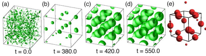
FIG. 6. (Color online) bcc structure obtained in the FitzHugh-Nagumo equation. (a)–(d) Structural evolution of domains for \beta = 0.09 , L = 0.198 = \delta x N with \delta x = 6.20 \times 10^{-3} and N = 32 , and \sigma = 1.0 \times 10^{-3} represented by the isosurface of u and (e) Bragg spots for I_k > 10^{-4} . The meanings of (e) are the same as those in Fig. 2. In order to make the initial randomness visible the domains in (a) represent the isosurface of u = 0.17468 whereas those in (b)–(d) represent the isosurface of u = 0.05 .
