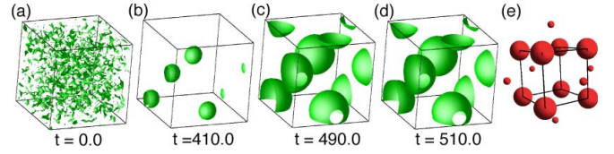
FIG. 7. (Color online) fcc structure obtained in the FitzHugh-Nagumo equation. (a)–(d) Structural evolution of domains for \beta = 0.09 , L = 0.128 = \delta x N with \delta x = 4.00 \times 10^{-3} and N = 32 , and \sigma = 1.0 \times 10^{-3} , represented by the isosurface of u and (e) Bragg spots for I_k > 10^{-4} . The meanings of (e) are the same as those in Fig. 2. The values of the isosurface are the same as those in Fig. 6.
