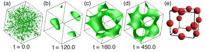
FIG. 12. (Color online) Single-gyroid structure obtained in the Brusselator (a)–(d) Structural evolution of domains for B=4.00 , L=0.124 = \delta x N with \delta x = 3.88 \times 10^{-3} and N=32 , and \sigma = 1.0 \times 10^{-2} , and (e) Bragg spots for I_k > 1.5 \times 10^{-4} . The meanings of (e) are the same as those in Fig. 2. In order to make the initial randomness visible the domains in (a) represent the isosurface of u=2.7002 whereas those in (b)–(d) represent the isosurface of u=2.7 .
