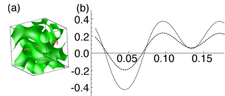
FIG. 3. (Color online) Spatial variation of the concentrations u and v for double-gyroid structure for \beta=0.05 , L=0.176=\delta x N with \delta x=5.53 \times 10^{-3} and N=32 , and \sigma=5.0 \times 10^{-3} . (a) The isosurface of u of double-gyroid structure. (b) Concentration of u (solid line) and v (dotted line) along the red arrow in (a).
