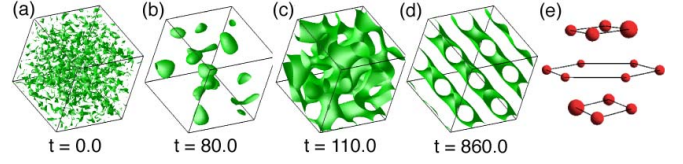
FIG. 5. (Color online) Perforated lamellar structure obtained in the FitzHugh-Nagumo equation. (a)–(d) Structural evolution of domains for \beta = 0.045 , L = 0.200 = \delta x N with \delta x = 6.25 \times 10^{-3} and N = 32 , and \sigma = 5.0 \times 10^{-3} , and (e) Bragg spots for I_k > 1.5 \times 10^{-4} . The meanings of (e) are the same as those in Fig. 2. In order to make the initial randomness visible the domains in (a) represent the isosurface of u = 0.08925 whereas those in (b)–(d) represent the isosurface of u = 0.05 .
