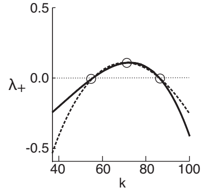
FIG. 15. Approximant for \lambda_+ . The dotted line is given by Eq. (A1) for D_u=2.0 \times 10^{-4} , D_v=1.6 \times 10^{-3} , A=2.7 , and B=4.0 . The solid line is the approximant given by Eq. (A9).
