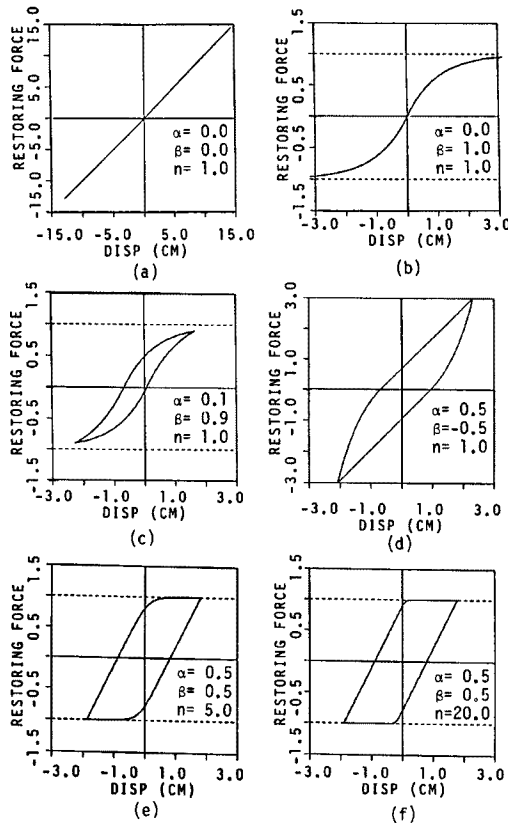
Fig. 16. Hysteretic restoring forces for various parameters.
