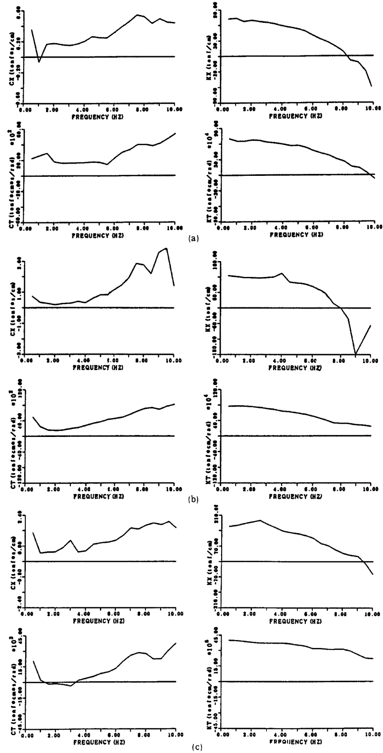
Fig. 8. Complex stiffness calculated by using the results of dynamic test.
