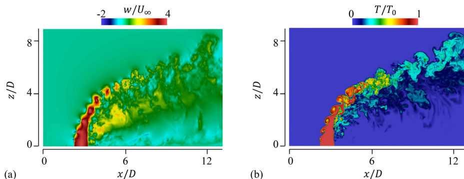
FIG. 26. Schematic of the DNS of a single jet issued into a crossflow.
