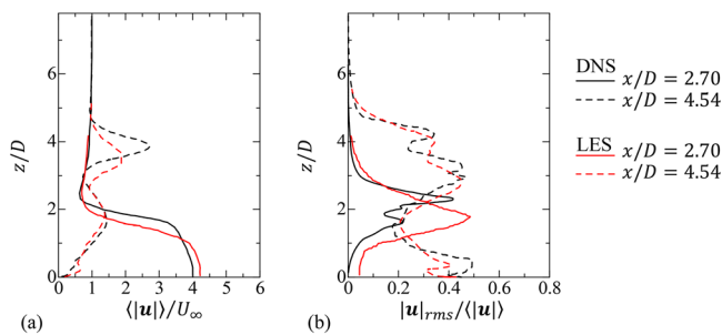
FIG. 28. Vertical profiles of (a) mean and (b) rms fluctuations of velocity magnitude at x/D = 2.70 and 4.54 . These results are compared with LES data. 22
