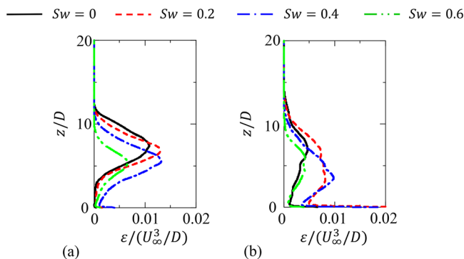
FIG. 23. Vertical profiles of the dissipation rate of turbulent kinetic energy \varepsilon . Panels show the profiles at different streamwise locations: (a) x/D = 20 and (b) x/D = 40 .
