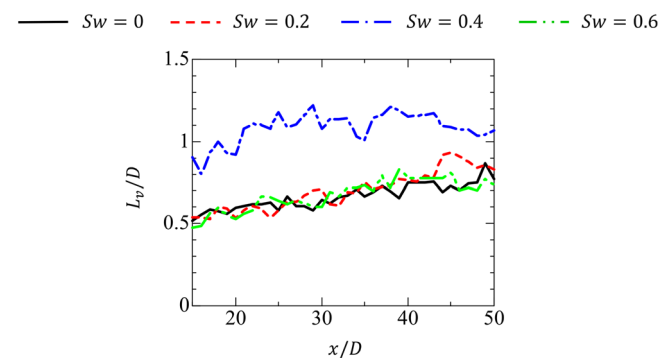
FIG. 24. Streamwise variations of the integral scale L_v in the fully developed jet region with spanwise homogeneity ( x/D \geq 15 ) at the vertical locations where the dissipation rate reaches the peak.
