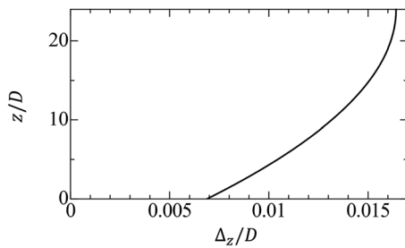
FIG. 3. Vertical distribution of vertical grid spacing \Delta z .
