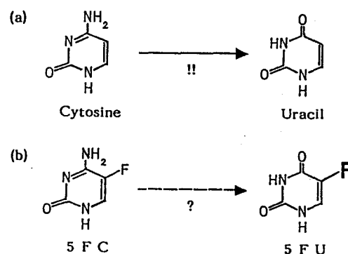
Figure 1-2. Cytosine deaminase.
