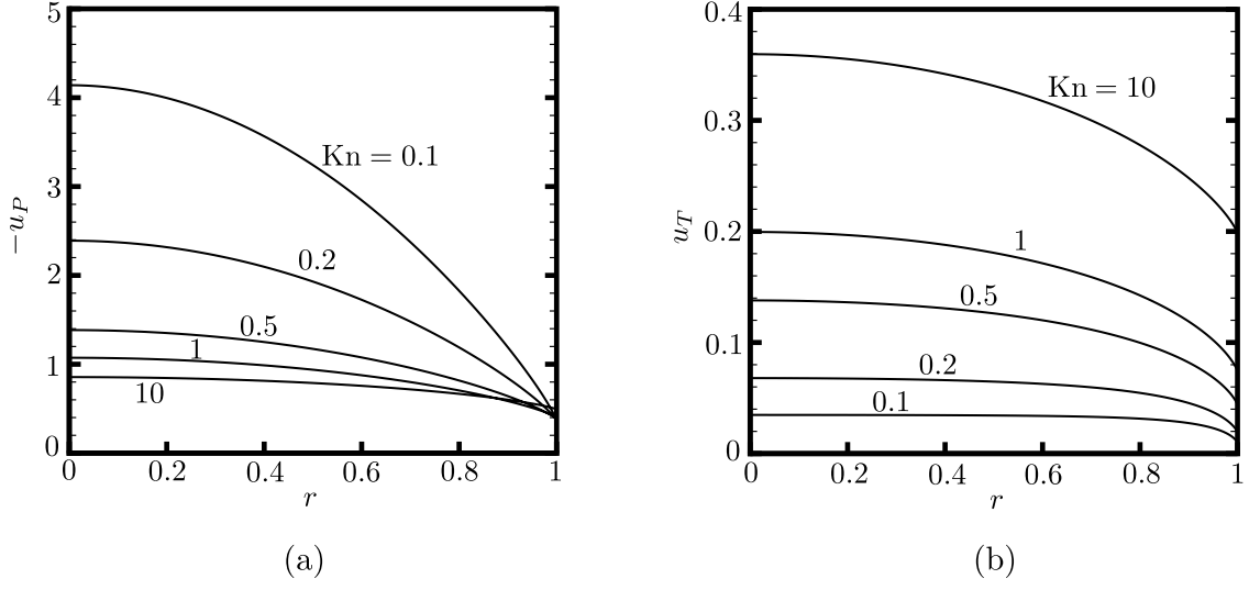
Figure 2.2: Profiles of the flow velocities for the Poiseuille flow and thermal transpiration through a circular tube. (a) Dimensionless flow velocity u_P for the Poiseuille flow. (b) Dimensionless flow velocity u_T for the thermal transpiration.
