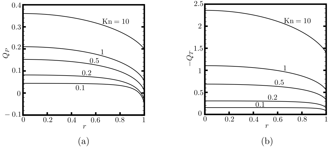
Figure 2.3: Profiles of the heat-flow vectors for the Poiseuille flow and thermal transpiration through a circular tube. (a) Dimensionless heat-flow vector Q_P for the Poiseuille flow. (b) Dimensionless heat-flow vector Q_T for the thermal transpiration.
