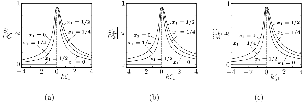
Figure 3.3: \tilde{\phi}_T^{(0)}/k versus k\zeta_1 at \zeta_\rho = 0.611 on three spatial points ( x_1 = 0, 1/4 and 1/2 ), where \zeta_\rho = (|\zeta|^2 - \zeta_1^2)^{1/2} . (a) k = 10 , (b) k = 10^2 and (c) k = 10^3 . Here, \tilde{\phi}_T^{(0)} \equiv \phi_T^{(0)} E^{1/2}/\zeta_2 is a function of x_1, \zeta_1 and \zeta_\rho .
