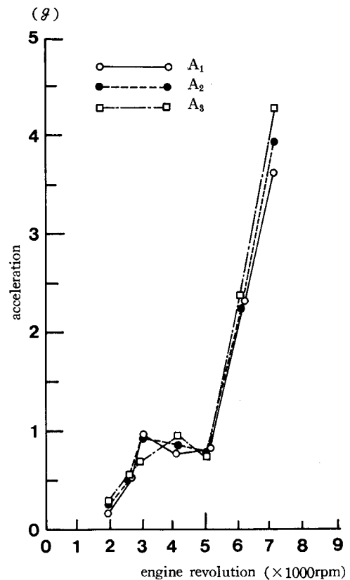
Fig. 5. The amplitudes of acceleration at the isolated chainsaw's handle. —the angle of the elbow ; 180° , tightly gripped—
