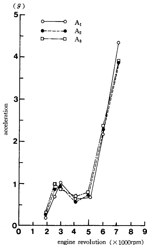
Fig. 6. The amplitudes of acceleration at the isolated chainsaw's handle. —the angle of the elbow; 90°, loosely gripped—
