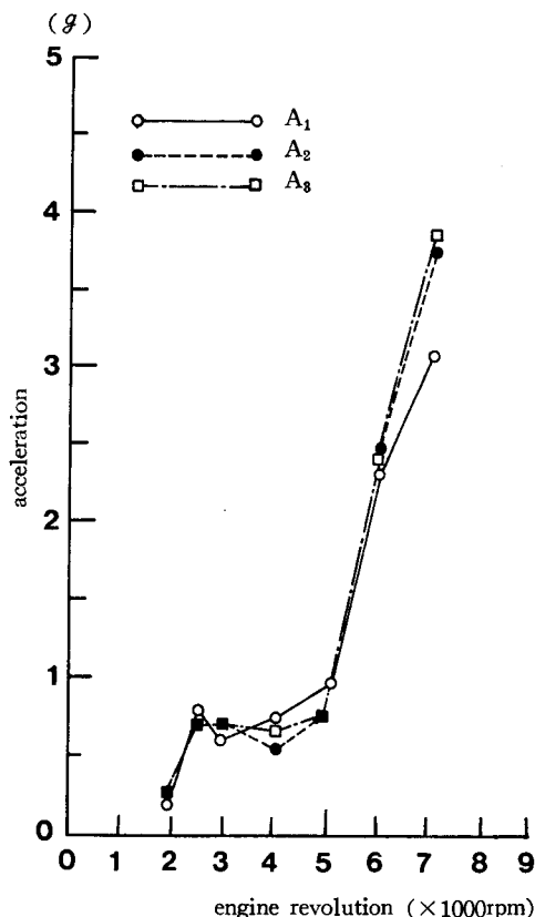
Fig. 7. The amplitudes of acceleration at the isolated chainsaw's handle. —the angle of the elbow; 90°, tightly gripped—
