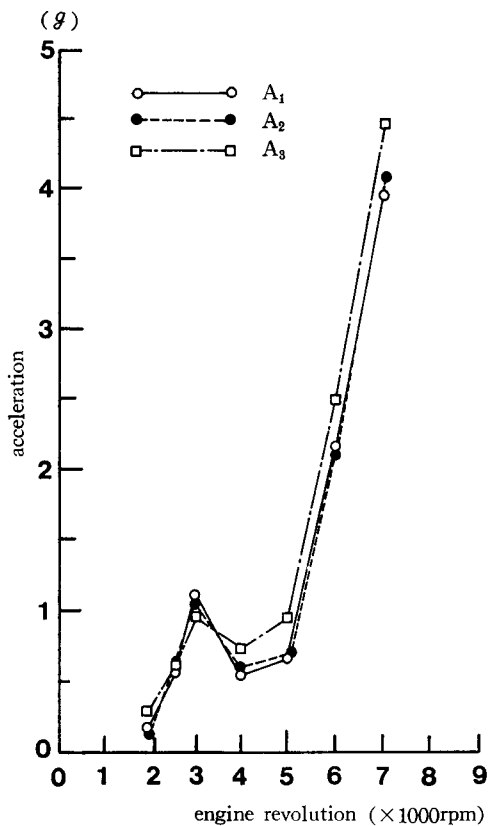
Fig. 4. The amplitudes of acceleration at the isolated chainsaw's handle. —the angle of the elbow ; 180° , loosely gripped—
