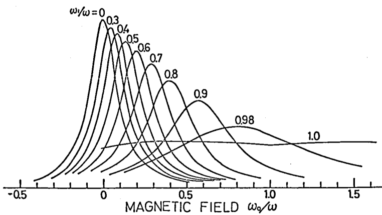
Fig. 3.13. Broadening and shift of the Hanle curve by the rotating rf field. Parameters for the theoretical curves: T = 0.01 sec, \omega = 1000 rad sec -1 and \theta = \pi/2 .
