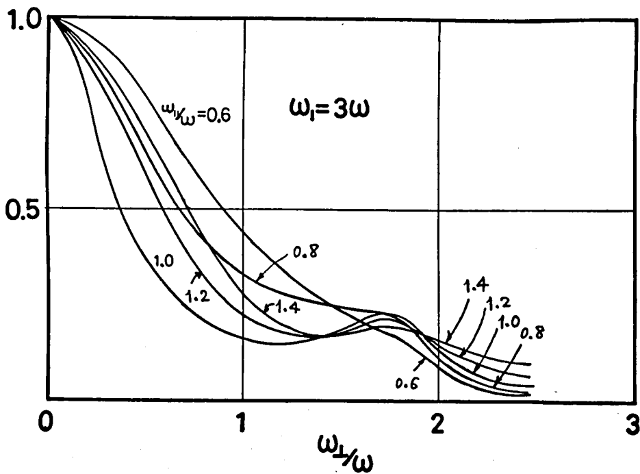
Fig. 5.26. Same as for Fig.5.25 but for \omega_{||} = 0.6\omega , 0.8\omega , \omega , 1.2\omega and 1.4\omega at \omega_1 = 3\omega . This figure is to be compared with the experimental results in Fig.5.19.
