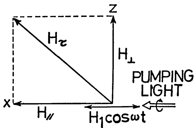
Fig. 5.12. This figure shows the directions of the magnetic fields and the pumping light beam to be considered in this section.
