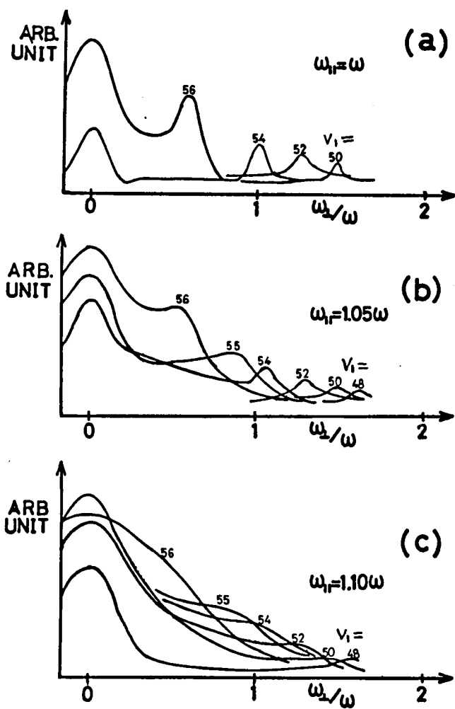
Fig. 5.19. Same as for Fig.5.18 but for \omega_{1r} = \omega ; (a), (b) and (c) are for \omega_{1r} = \omega , 1.05\omega and 1.10\omega , respectively.
