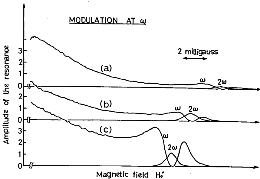
Fig.3.10. Resonance curves in the component modulated at \omega ; (a), (b) and (c) correspond to the cases that the intensity of H_1 is small, medium and large, respectively. The resonance curves in the component modulated at 2\omega are also shown.
