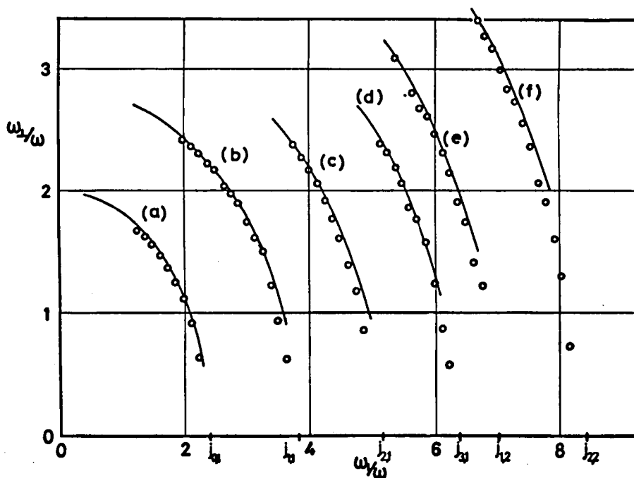
Fig. 5.28. Positions of the various Haroche like resonances as a function of \omega_1 ; (a) is the first Haroche resonance, (b), (c) and (d) are the first Haroche like resonances for \omega_{//} = \omega, 2\omega, 3\omega , respectively. (e) and (f) are the second Haroche like resonances for \omega_{//} = \omega, 2\omega , respectively. The encircled points are the experimental results and the solid lines show the numerical results. It should be noticed that the values of \omega_1/\omega , at which the Haroche like resonances for \omega_{//} = q\omega enter the zero field of H_1 , corresponding to the values at the zeros of the q -th order Bessel function J_q(\omega_1/\omega) . The values of J_{n,m} 's represent the m -th zero of the n -th order Bessel function J_n(\omega_1/\omega) .
