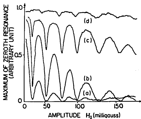
Fig. 4.7. Level crossing curves as a function of H_1 for various values of h . Recorder traces showing the variation of the maximum of the zeroth resonance due to the amplitude H_1 . The amplitude h is varied as a parameter; (a), (b), (c) and (d) are the cases that h = 0.7 milligauss, 2.0 milligauss, 6.2 milligauss and 18.2 milligauss, respectively.
