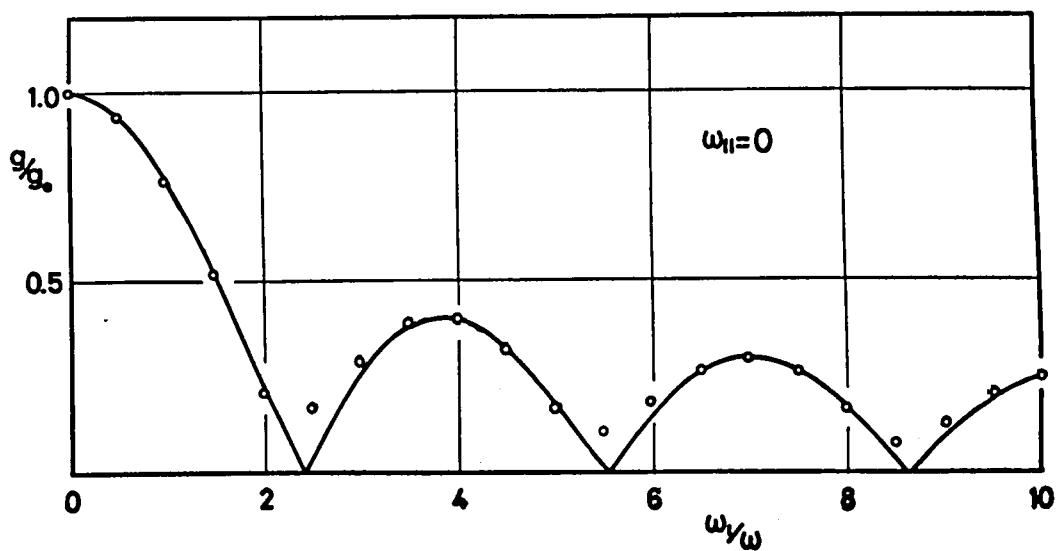
Fig. 5.21. Effective g -factor derived from the width of the Hanle curves in Fig.5.20. The computational results derived from Fig.5.20 are represented by the encircled points and the zeroth-order Bessel function as a function of \omega_1/\omega is represented by the solid line for comparison.
