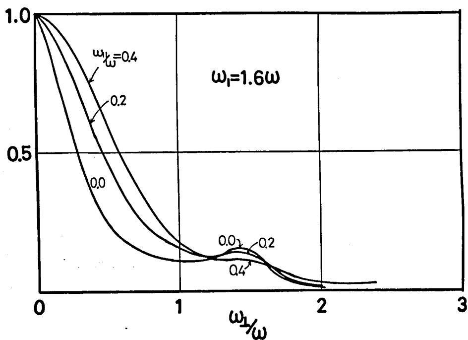
Fig. 5.25. Behavior of the Haroche like resonance near \omega_{II} = 0 .
