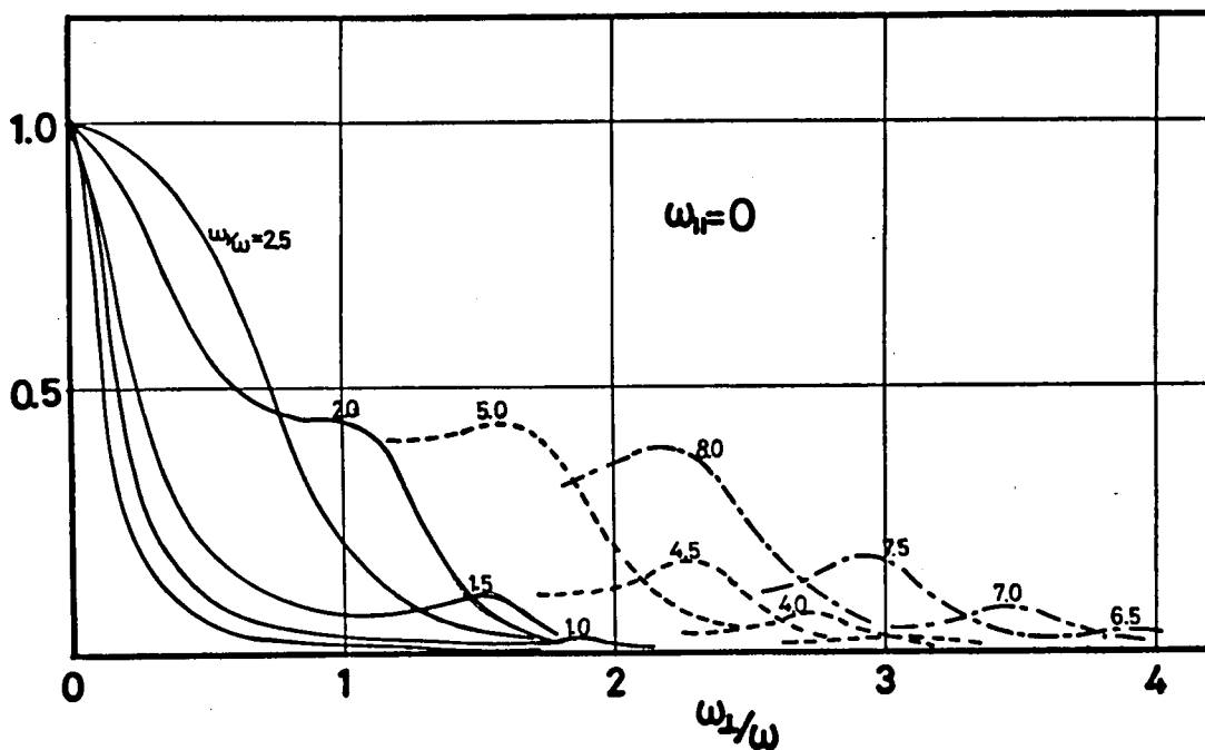
Fig. 5.20. Numerical result to be compared with Fig. 5.13, in which the Haroche resonance for \omega_H = 0 obtained in experiment is shown. The solid lines show the first Haroche resonance and the Hanle curve as a function of \omega_L/\omega . The dashed lines and the dotted broken lines show the second and the third Haroche resonances, respectively.
