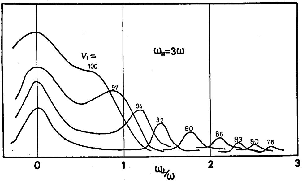
Fig. 5.17. Same as for Fig.5.15 but for \omega_{//} = 3\omega .
