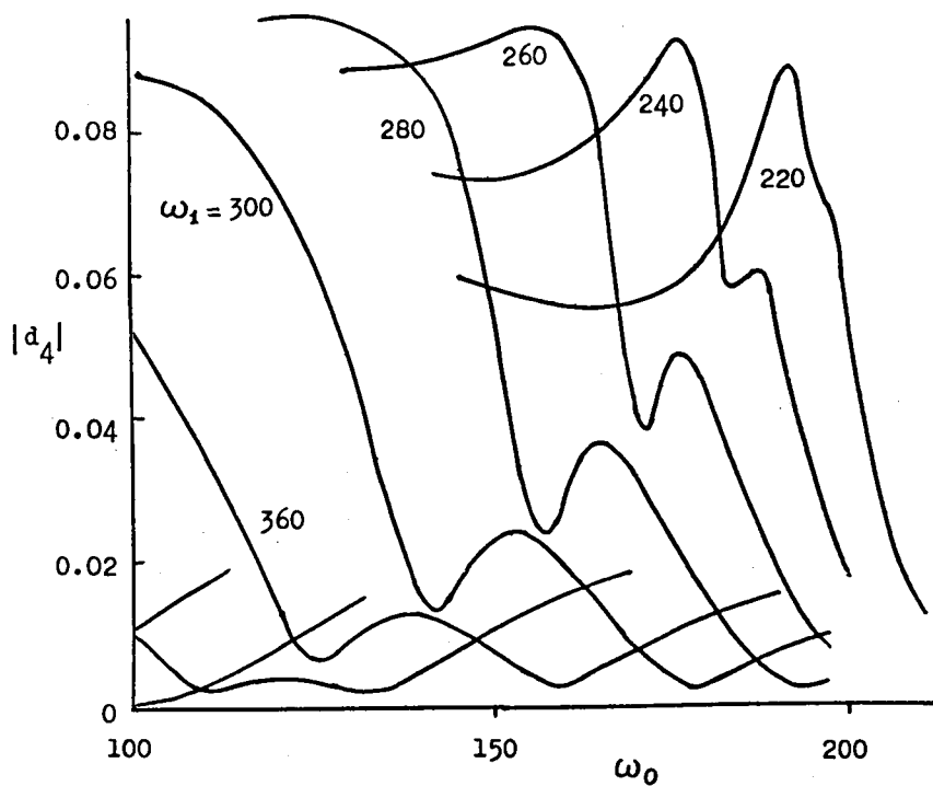
Fig. 5.10. (b). Theoretical curves for the component modulated at 4\omega .
