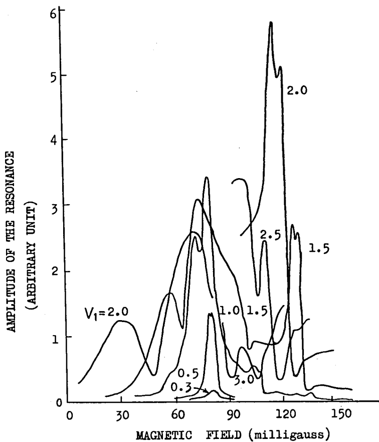
Fig. 5.9. (b). Experimental recordings for the resonances at \omega_0 = 3\omega and \omega_0 = 5\omega in the component modulated at 4\omega . Experimental condition: \omega / 2\pi = 5 \text{ KHz} .
