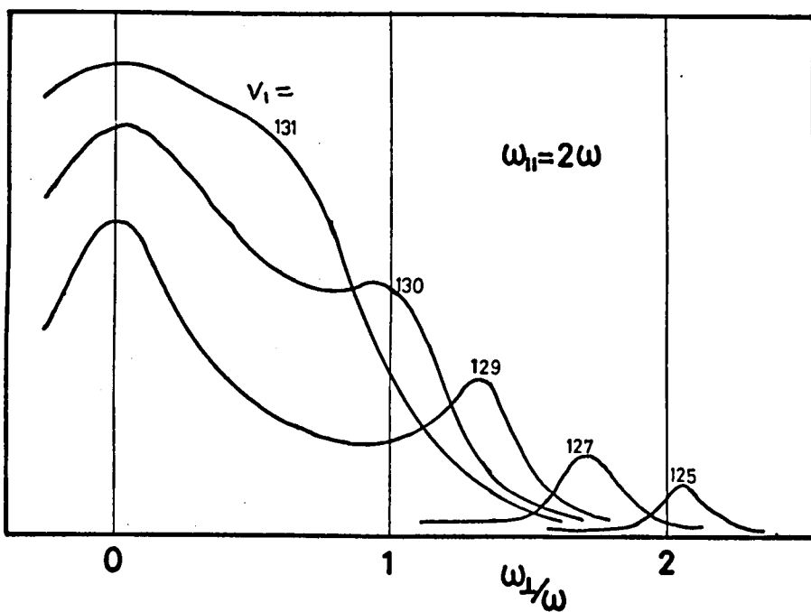
Fig. 5.16. Same as for Fig. 5.15 but for \omega_{||} = 2\omega ; (a) and (b) show the first and the second Haroche like resonances, respectively.
