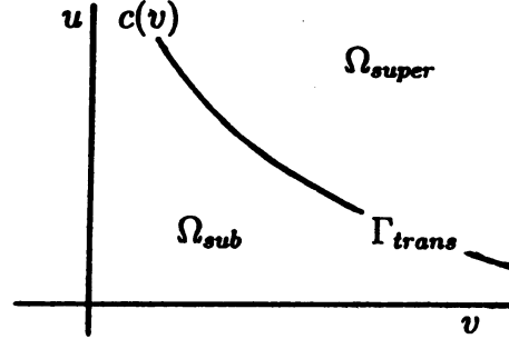
Figure 1.1( \gamma > 1 )
