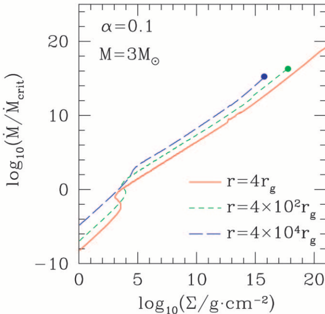
FIG. 5.—Thermal equilibrium curves on the (\Sigma, \dot{M}) plane at r = 4r_s (solid line), 400r_s (dashed line), and 4 \times 10^4 r_s (long-dashed line). All other parameters are the same as in Fig. 4. The solid circles at the upper ends indicate the location of H = r , above which no physical solution exists.
