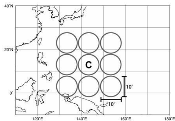
Fig. 7 Nine circles to calculate upper tropospheric circulation. A diameter of each circles is 1,387 km. “C” is a genesis location of averaged for all 904 tropical cyclogenesis cases for 30 years.
