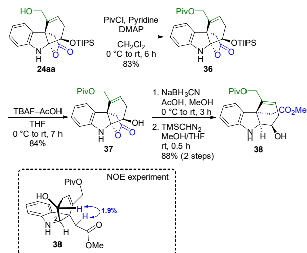
Scheme 8. Reductive Ring-Opening Reaction Starting from 24aa
