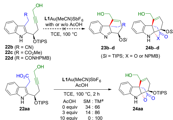
Scheme 4. Effect of the Substrate Structure and Acid on the Reaction
