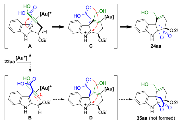
Scheme 7. Reaction Stereoselectivity
