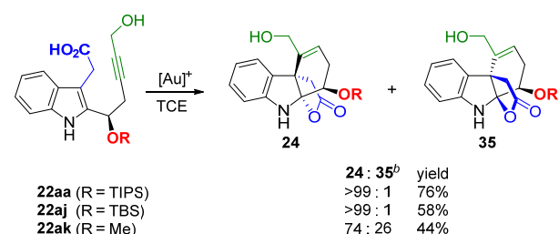
Scheme 6. Effect of an Oxygen-Protecting Group on the Reaction Stereoselectivity a
