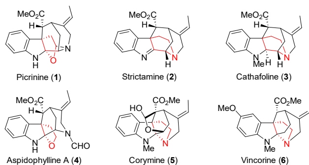
Figure 1. Representative akuammiline alkaloids.
