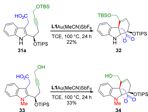
Scheme 5. Effect of the Free Hydroxy Group and NH Indole
