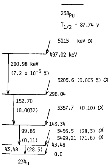
Fig. 1. Decay scheme of ^{238}\text{Pu} and ^{234}\text{U} 43.48 keV state.
