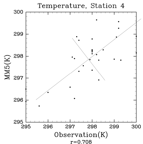
Fig. 4 Scatter diagram of the day-to-day variations of the daily averaged surface temperature in August 2004 at Station No. 4 between the observation and the MM5 output.
