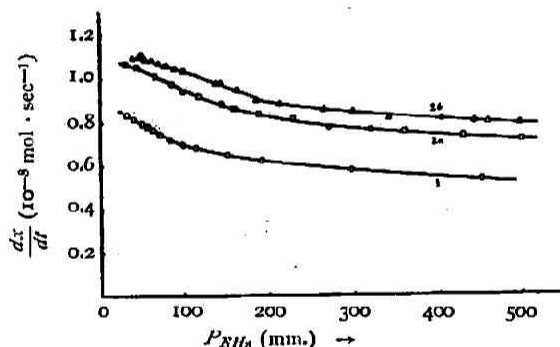
Fig. 8. The change of the decomposition velocity (the relative quantum yield) with ammonia pressure.
