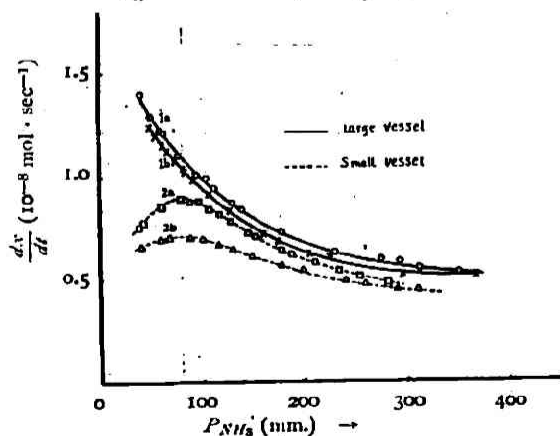
Fig. 7. Homogeneous reaction velocity.
