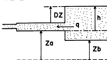
Fig. 4 Formulation of lava flow over the topography digitized with the interval, W (representation in the vertical cross-section). q is the flow rate of lava through the boundary of a mesh. \rho and \eta are the density and the viscosity of lava. g is the acceleration due to gravity.
