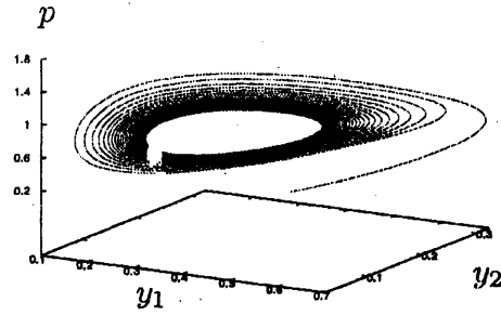
Figure 2: Limit cycle with \epsilon = 3
