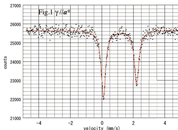
Fig.1 shows representative Mössbauer spectrum of enstatite measured under incident \gamma -ray parallel to a^* -axis. A doublet due to Fe 2+ in M2 site of orthopyroxene was observed. Isomer shift, Q-splitting, and line width were 1.06 2.11 and 0.34 mm/s, respectively. From nine sets of intensity of quadrupole doublet, three components of traceless tensor were calculated as 0.116, -0.045 and -0.075. Asymmetric parameter \eta was 0.266.
