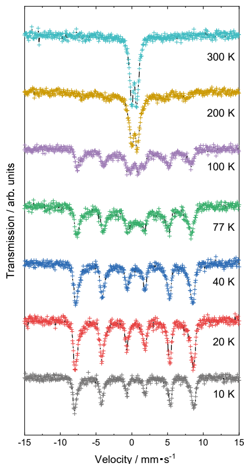
Fig. 1. Temperature dependence of Mössbauer spectra for (\text{Fe}_2\text{O}_3)_{0.5}(\text{Al}_2\text{O}_3)_{0.5} .
