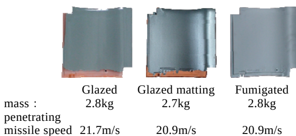
Photo 5 Roof tiles (JIS,J-type)
