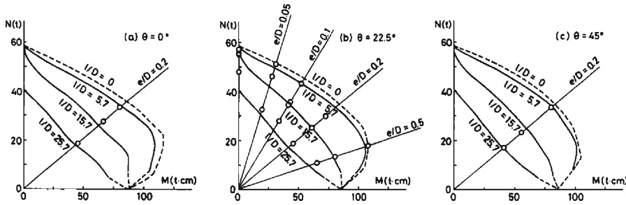
Fig. 13 Square long column interaction diagrams (units: 1t = 9.8 \text{ kN} , 1t \cdot \text{cm} = 0.098 \text{ kN} \cdot \text{m} ).
