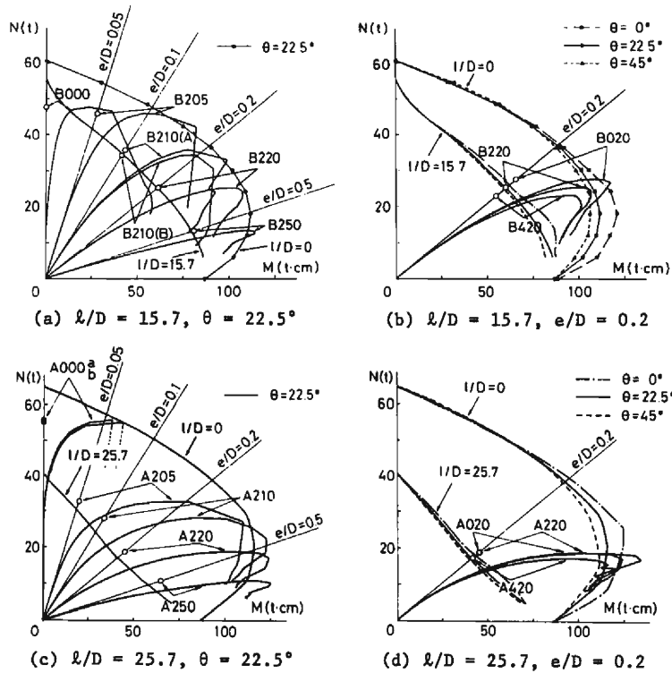
Fig. 12 Interaction diagrams for column section illustrating load-moment behavior up to failure (units: 1\text{ t} = 9.8\text{ kN} , 1\text{ t}\cdot\text{cm} = 0.098\text{ kN}\cdot\text{m} ).
