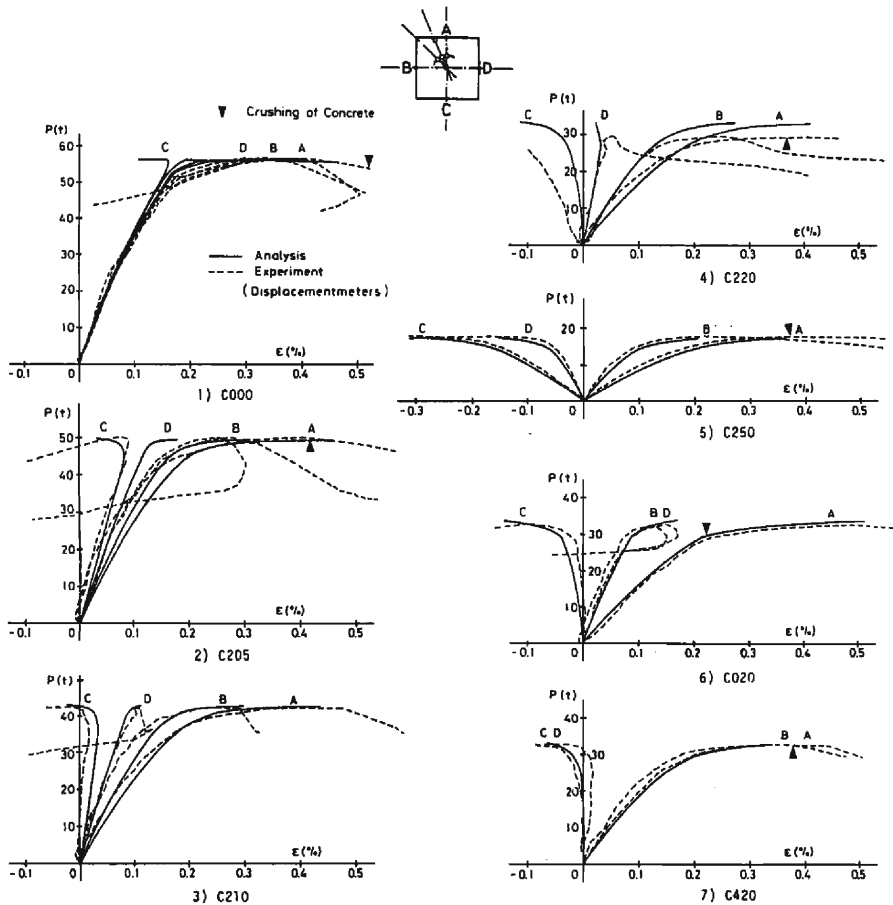
Fig. 7 Load versus longitudinal strain relationships (C series) (unit: 1t=9.8\text{ kN} ).
