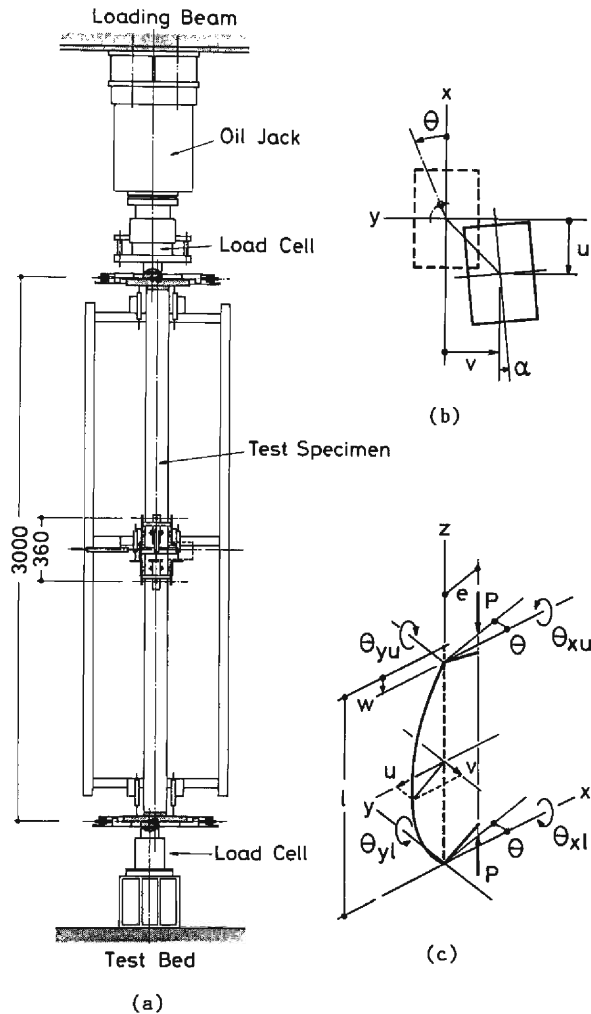
Fig. 2 Specimen in loading apparatus (units in mm).
