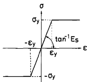
(b) Reinforcing Bar
