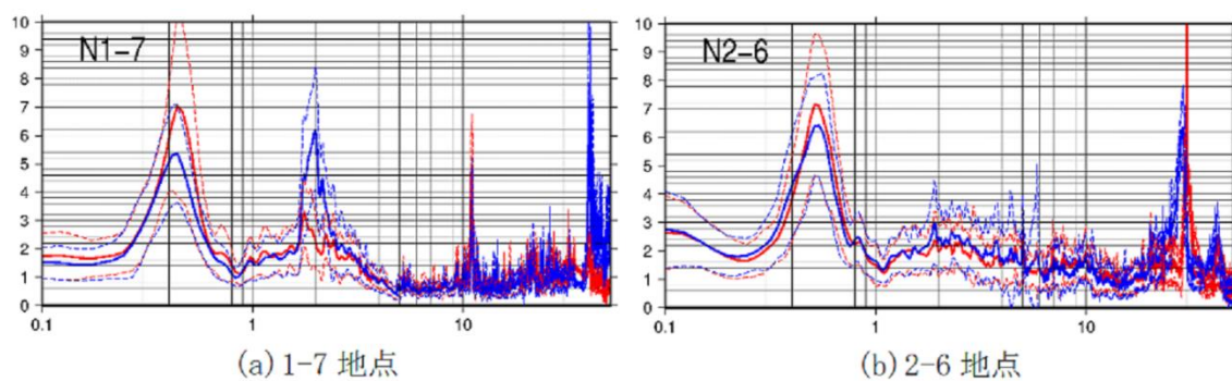
Fig. 16 Examples of observed MHVRs (blue: NS/UD, red: EW/UD) [CTOC09]
