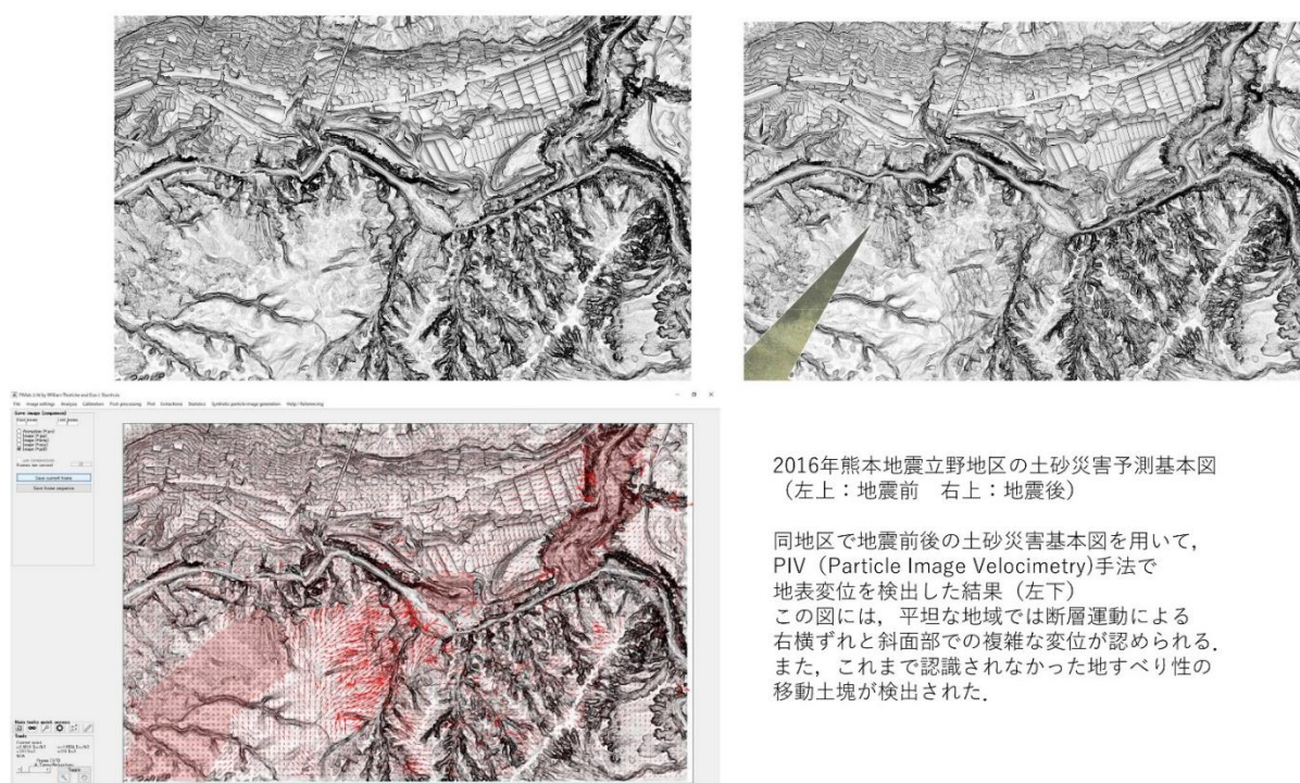
Fig. 8 Detection of surface displacement in the Tateno district during the 2016 Kumamoto Eq. [CTOC14]
