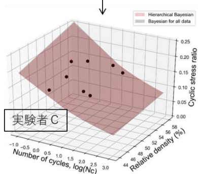
Fig. 2 Assessment of “uncertainty” of liquefaction characteristics from laboratory tests [CTOC01]
