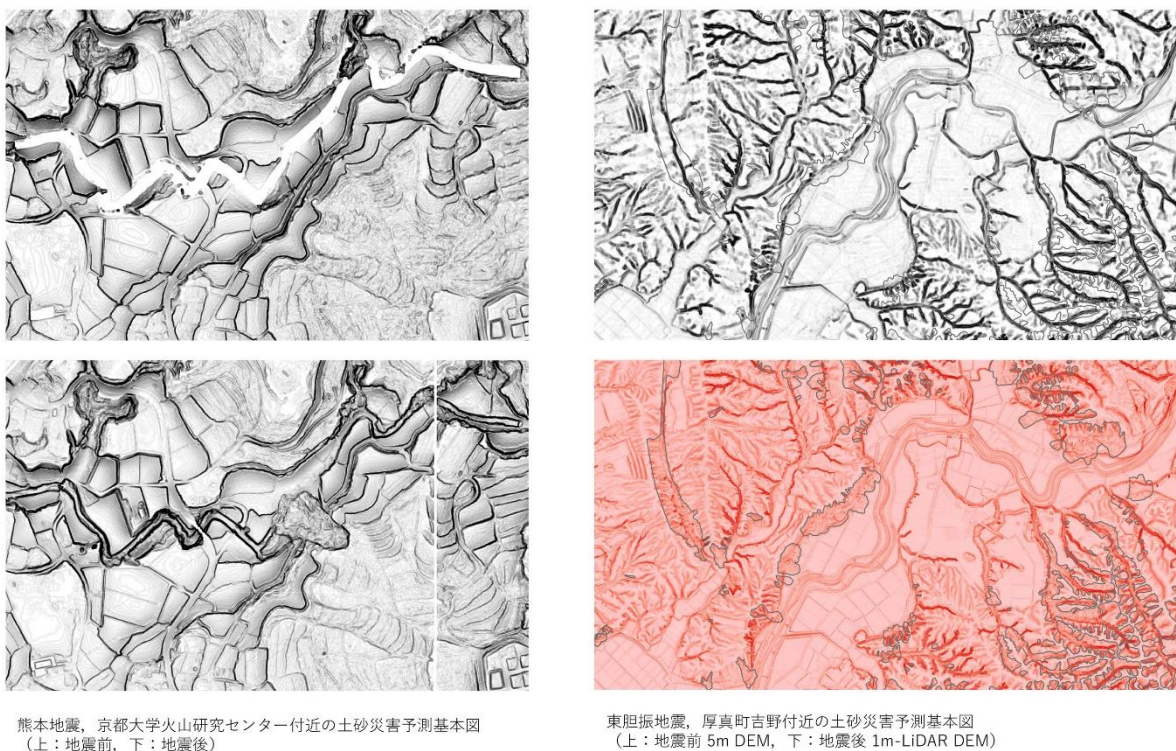
Fig. 7 Comparison of geomorphic feature map for forecasting landslides before and after earthquakes (left: 2016 Kumamoto Eq., right: 2018 Hokkaido Eastern Iburi Eq. [CTOC14])
