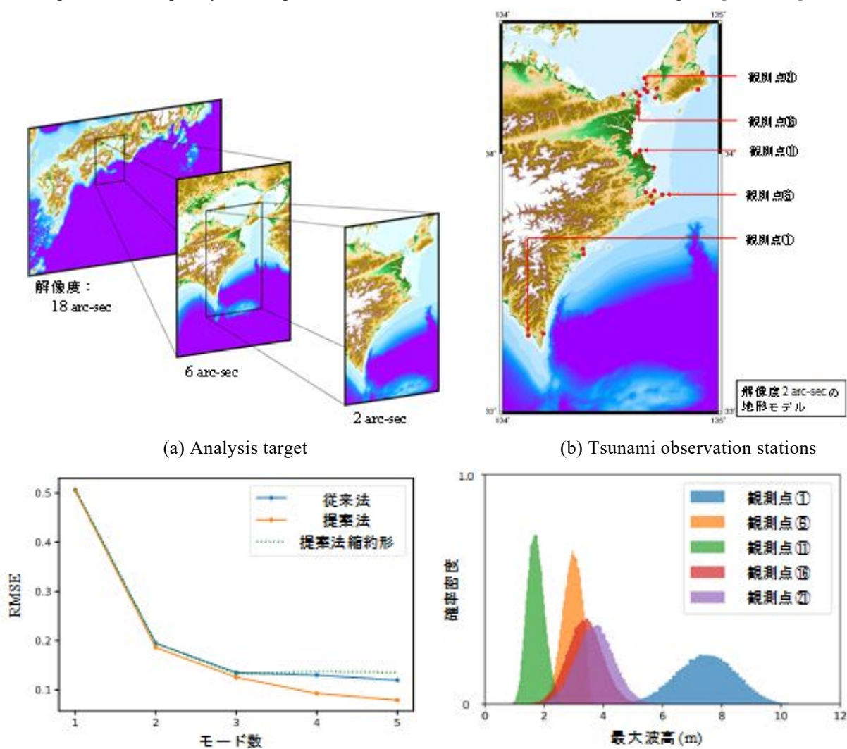
Fig. 18 Comparison of results obtained from combining the surrogate model and numerical analysis proposed by this study and the conventional method [CTOC18]
