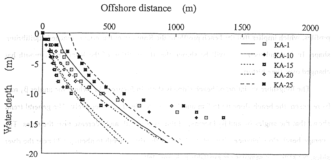
Figure 3.16 Variation of beach profiles along Kamo Delta coast compared with Dean's relationship for equilibrium beach profile.
