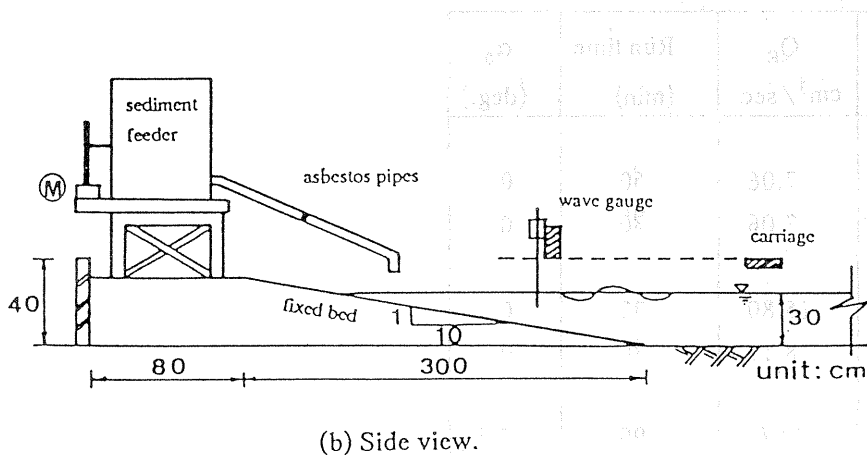
Figure 3.46 Schematic diagram of experimental arrangement of formation of river delta process.
