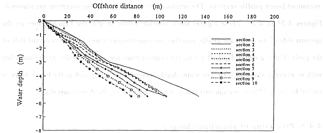
Figure 4.24 Variation of beach profiles along a stable beach between grain No. 11 and groin No. 15.
