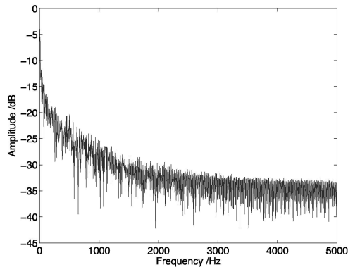
(b) Output voltage
