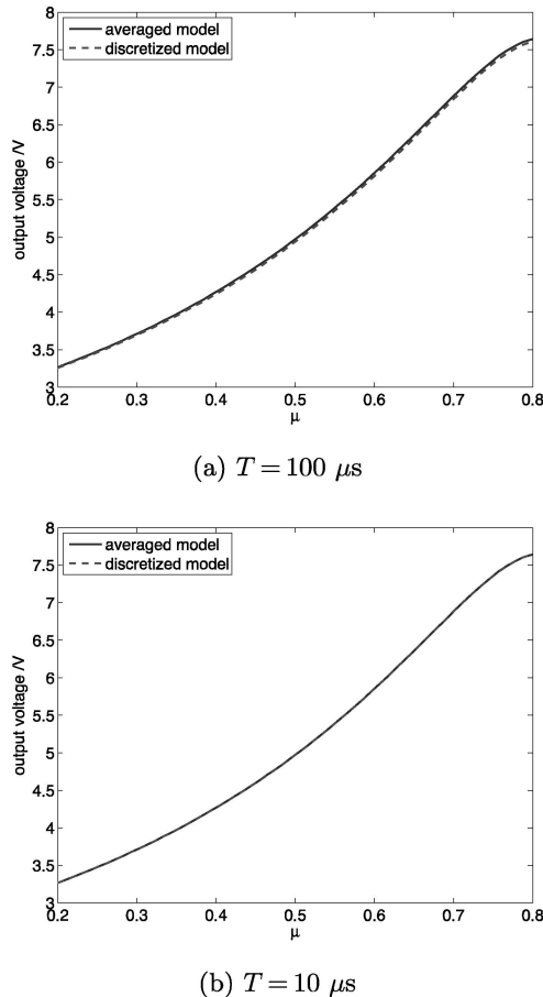
Fig. 3 Comparison of steady-state output voltage
