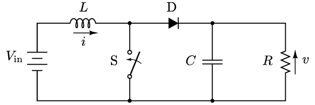
Fig. 1 Boost converter
