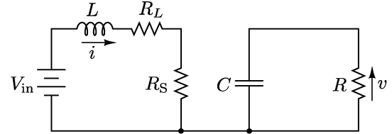
(a) Switch: ON
