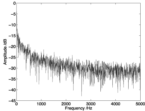
(a) Input signal
