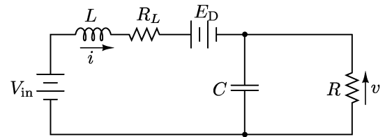
(b) Switch: OFF
