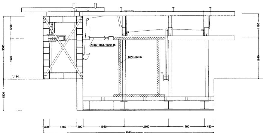
(a) Elevation
